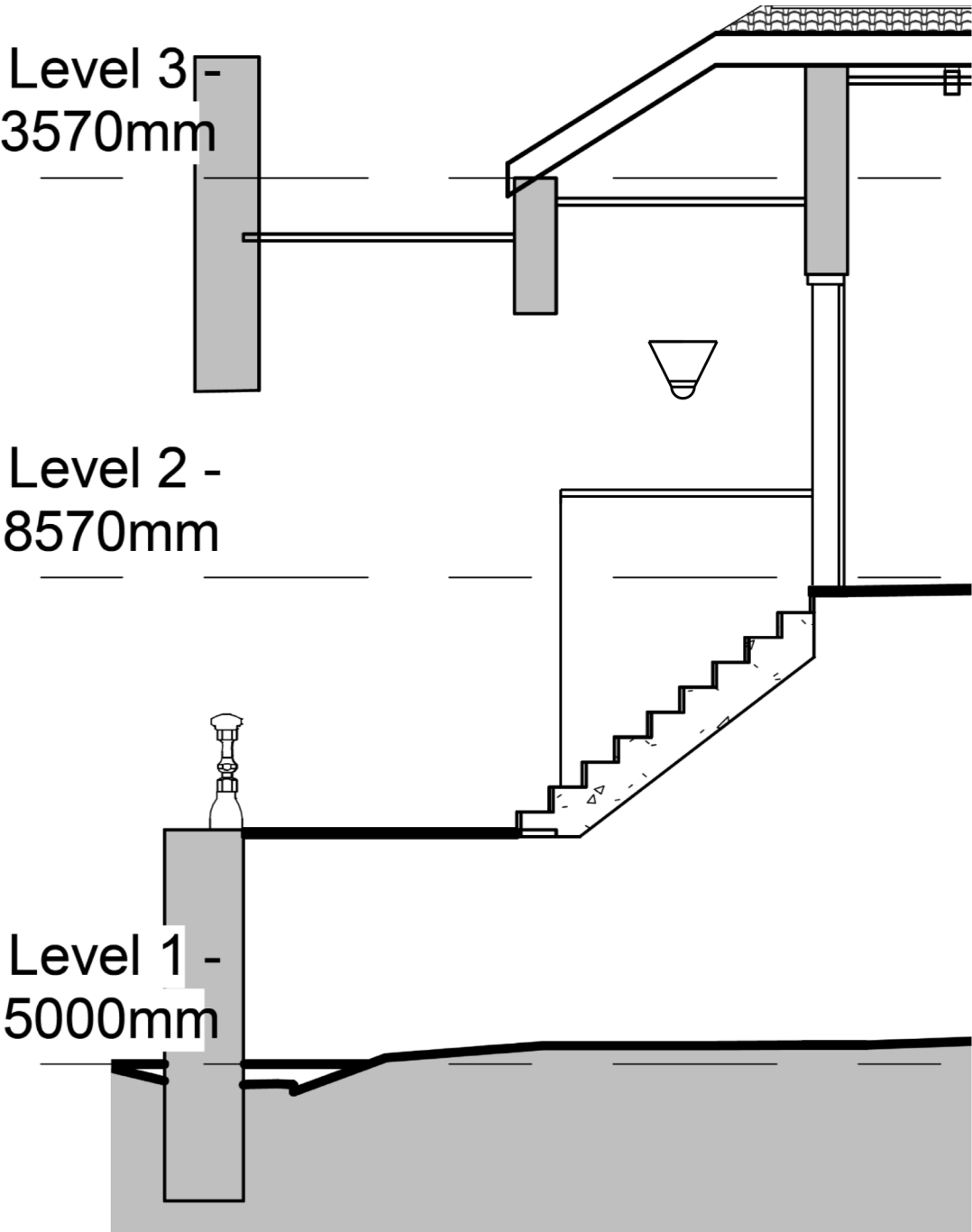
EXISTING ELEVATION 01 LEFT-HAND SIDE WALL TO THE ENTRANCE DOOR
