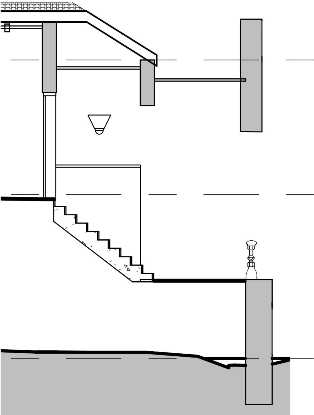
EXISTING ELEVATION 02 RIGHT-HAND SIDE WALL TO THE ENTRANCE DOOR
