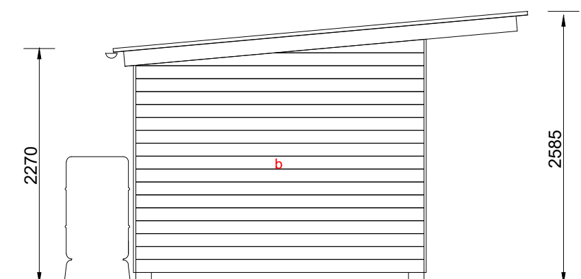
SIDE ELEVATION D
