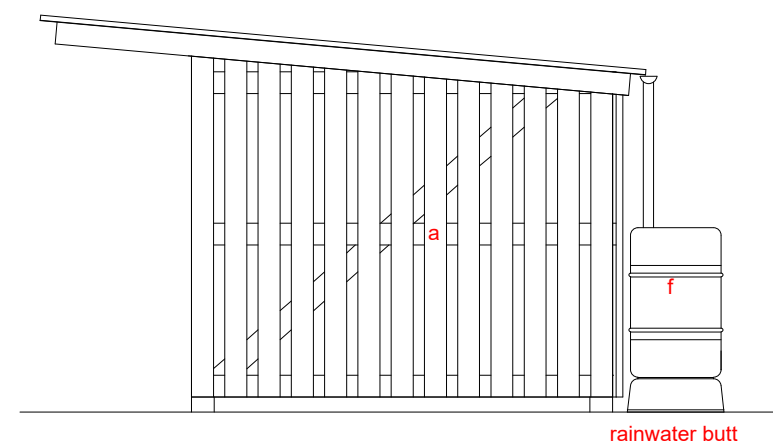
SIDE ELEVATION C
