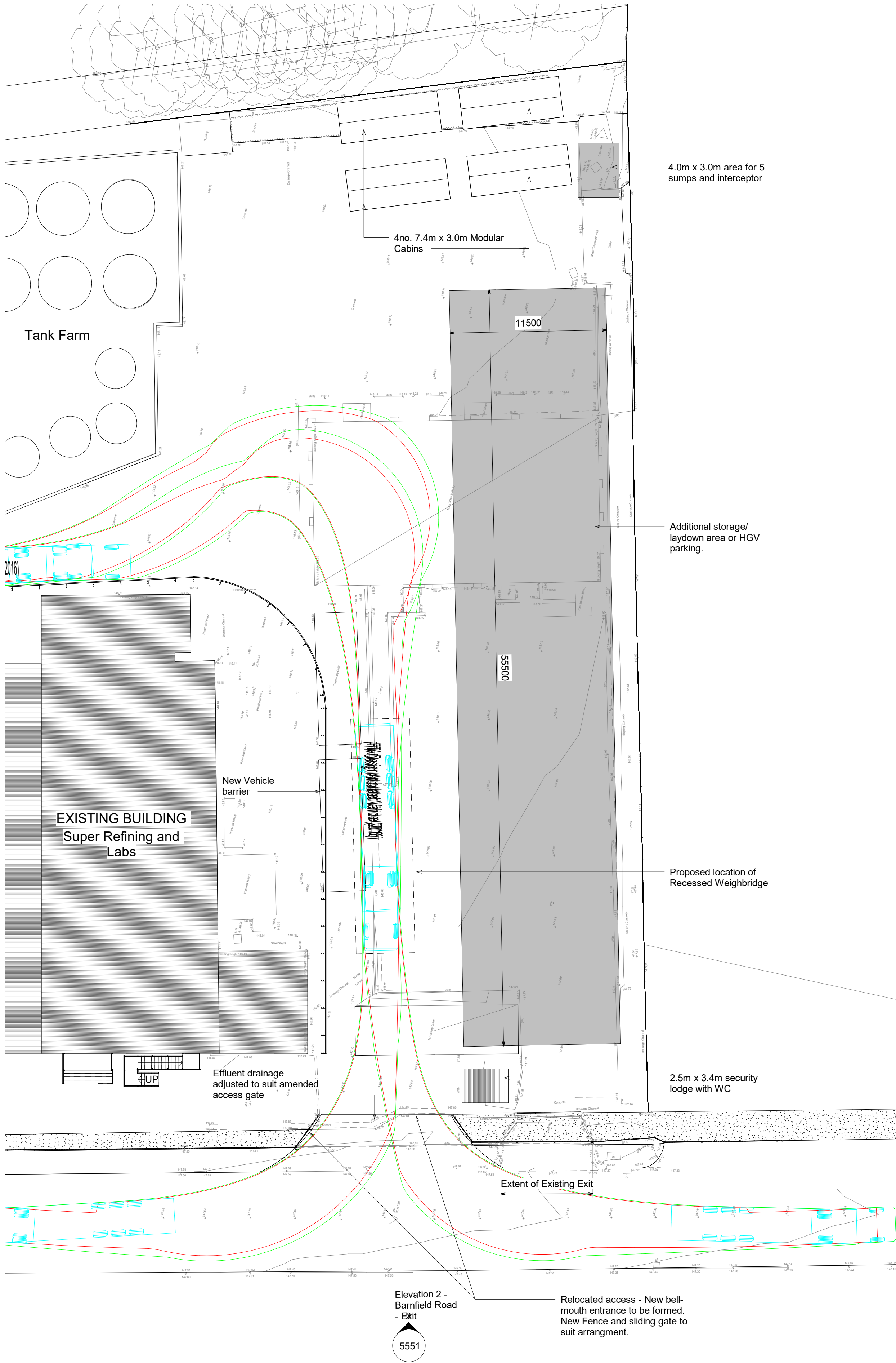
1 Entrance/ Exit Works - Exit Plan 1 : 200
