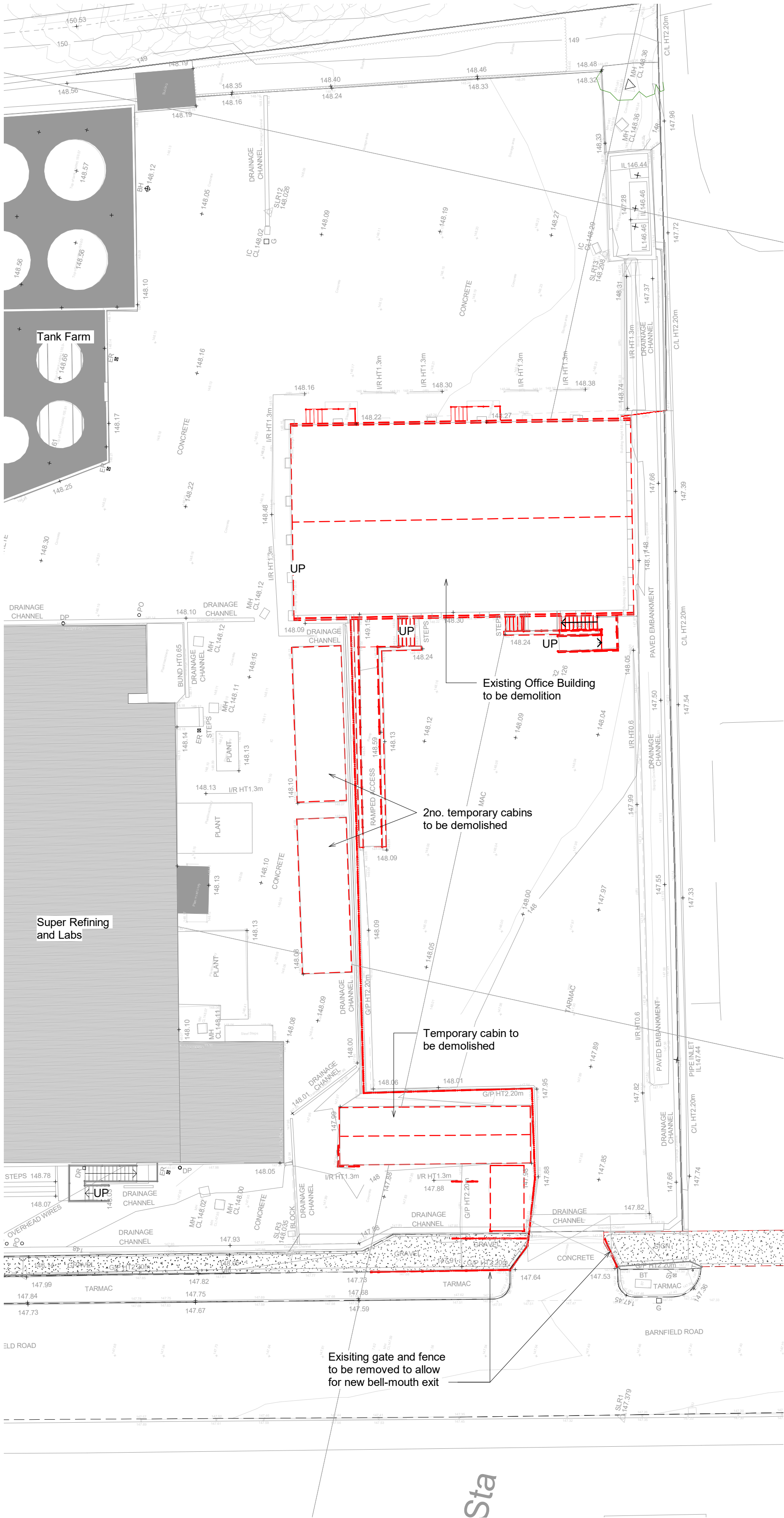
1 Entrance/ Exit Works - Exit Plan - Demolition 1 : 200
