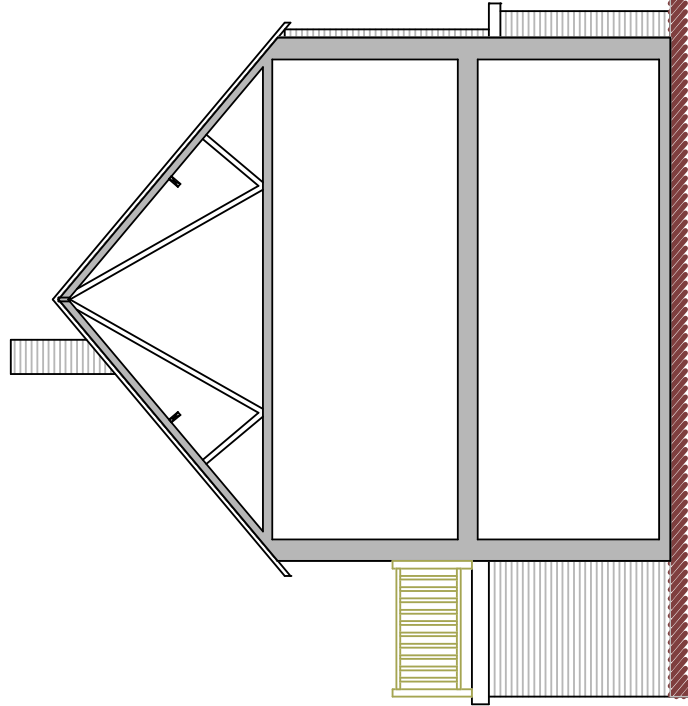
Side Elevation/Partial Section
