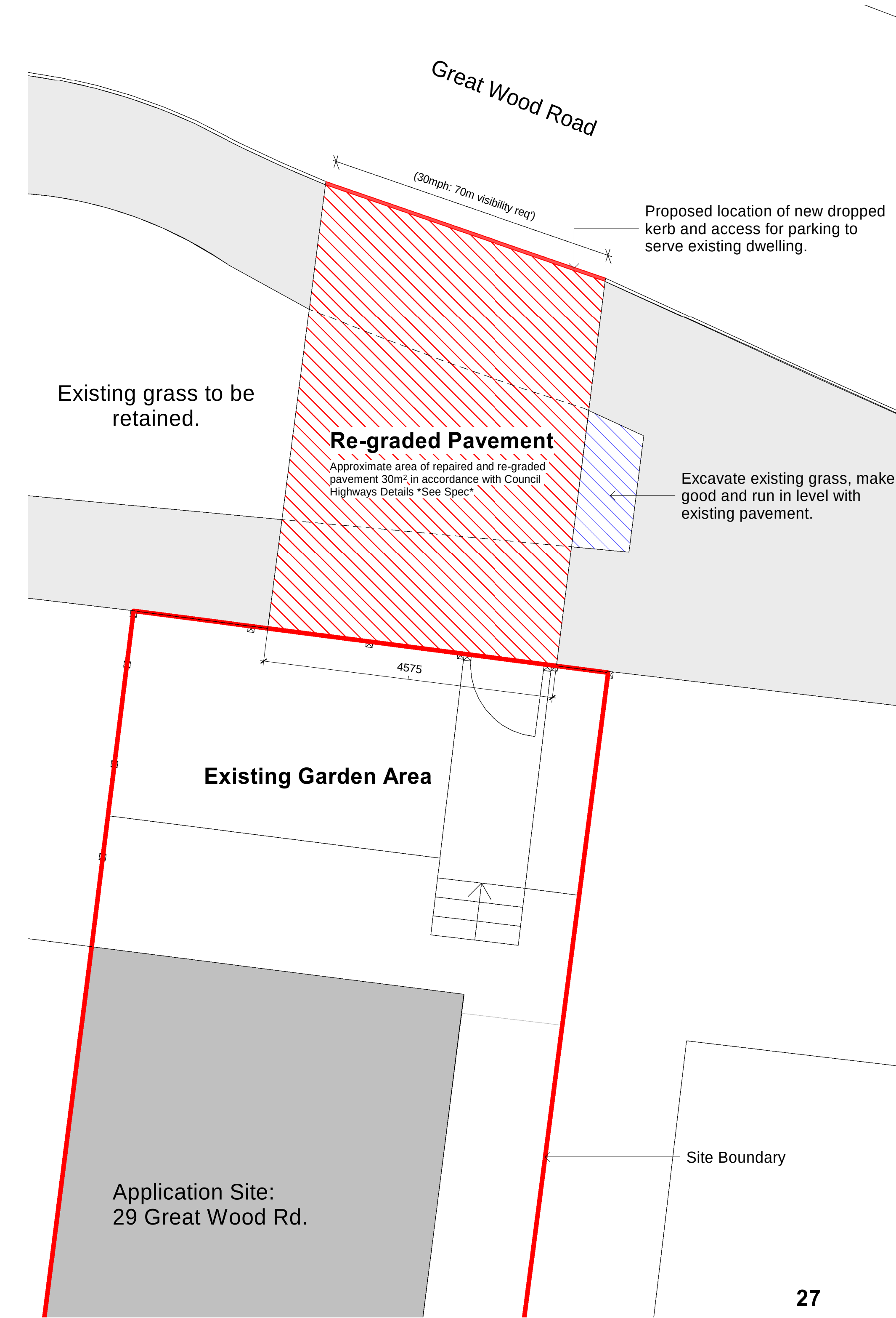
Proposed Block Plan 1 : 50
