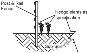
Fence Type 2 - Hedge / Fence Cross Section - 1:100 @ A3
