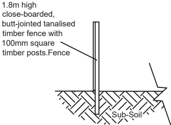
Fence Type 1 - Garden Fence Cross Section - 1:100 @ A3
