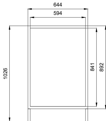
FRONT ELEVATION 1:20
