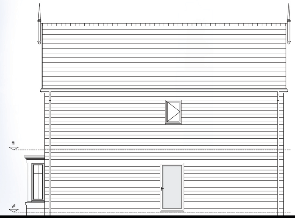
Rear Elevation
