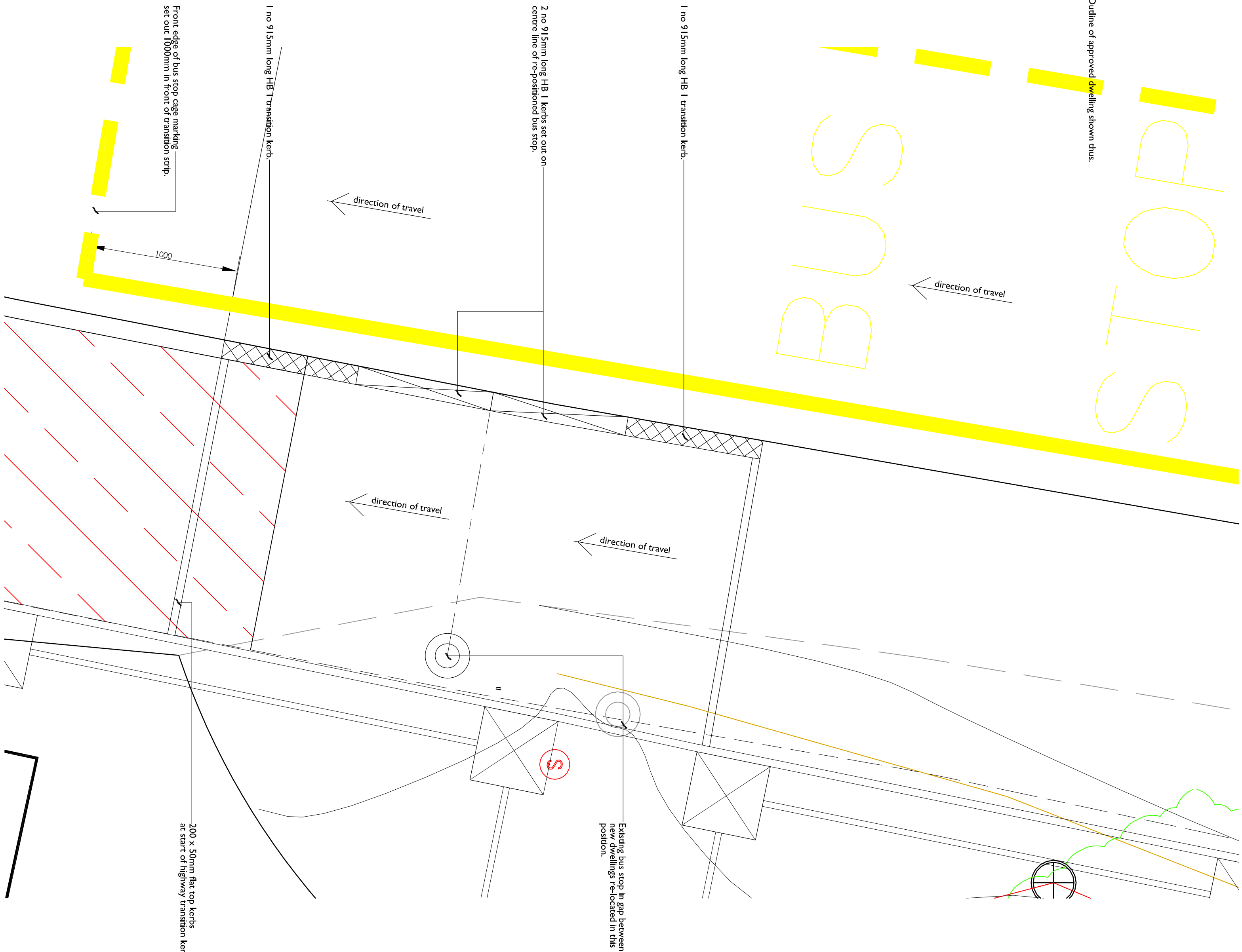
Detail of Bus Stop area set out scale: 1:20 at A1
