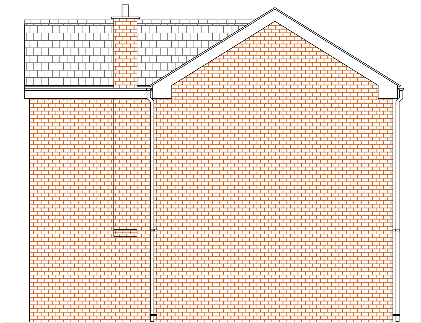
3 NORTH FACING ELEVATION 1:50 SCALE
