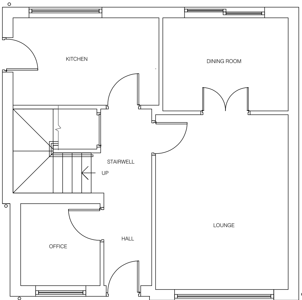
1 GROUND FLOOR PLAN - 51sqm 1:50 SCALE
