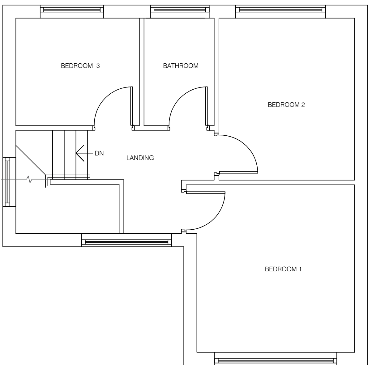
2 FIRST FLOOR PLAN - 42sqm 1:50 SCALE
