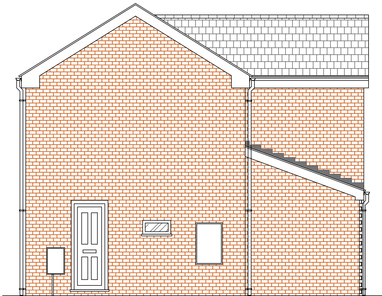
6 SOUTH FACING ELEVATION 1:50 SCALE
