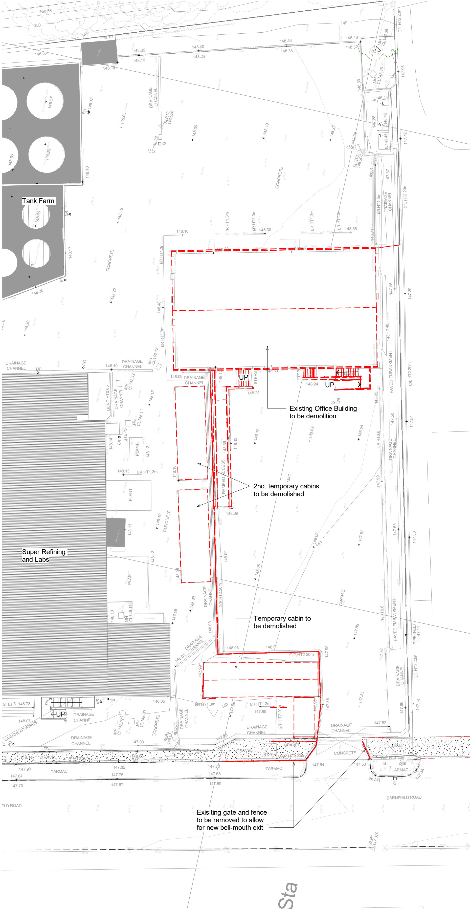
1 Entrance/ Exit Works - Exit Plan - Demolition 1 : 200
