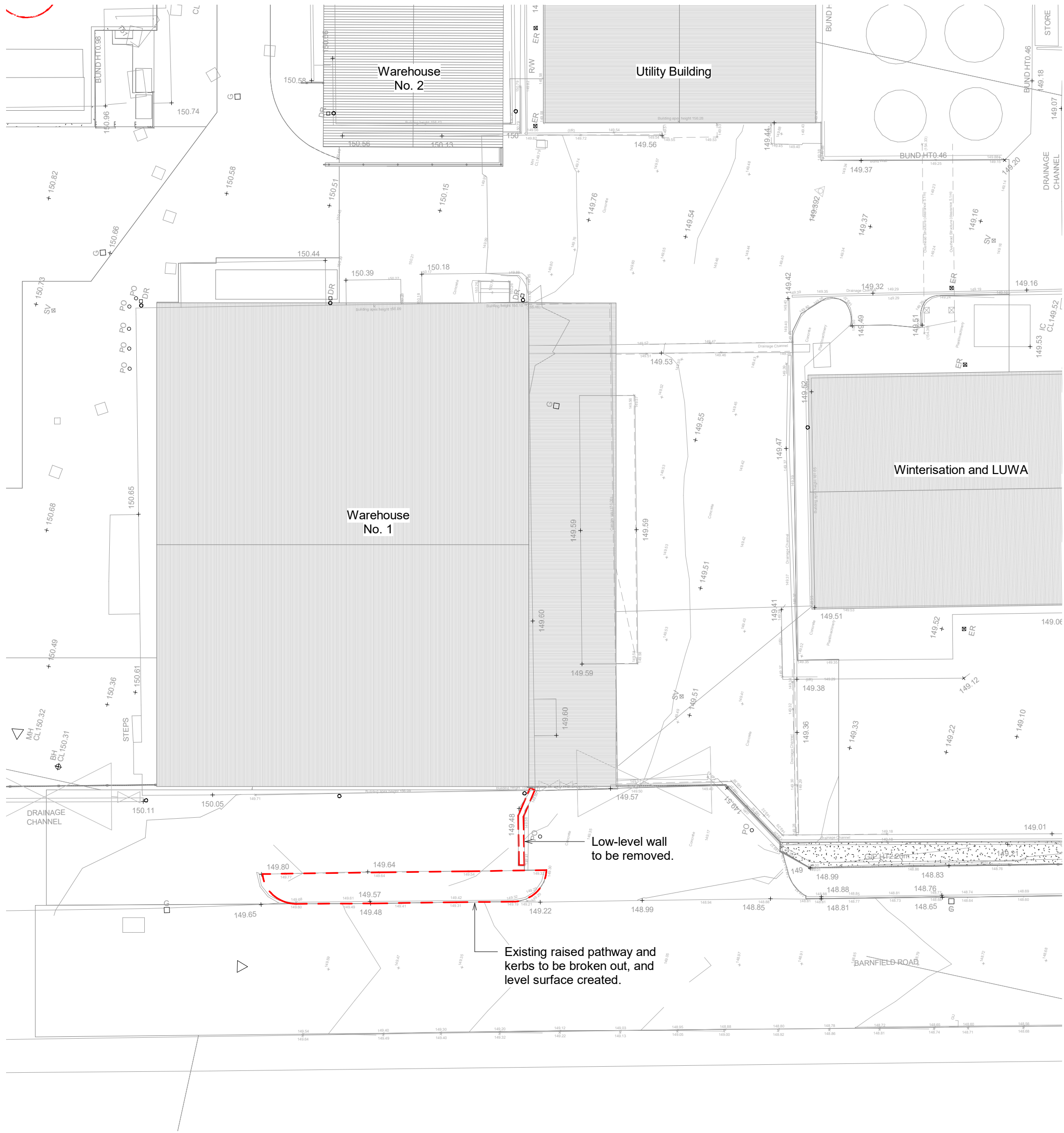
2 Entrance/ Exit Works - Entrance Plan - Demolition 1 : 200
