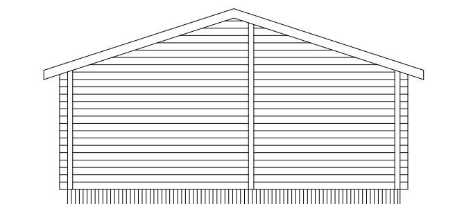
PROPOSED REAR ELEVATION SCALE - 1:100
