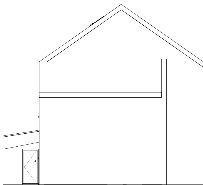
Existing Right Side Elevation 1 : 100
