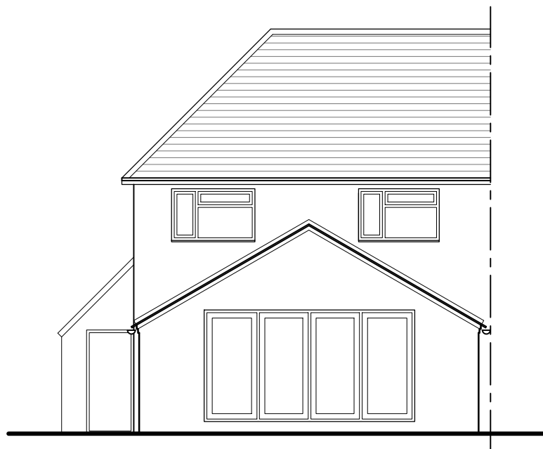
Rear Elevation (North)
