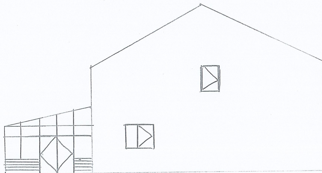
PROPOSED LEFT ELEVATION
