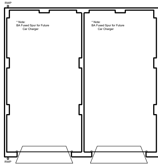
TWIN GARAGE
