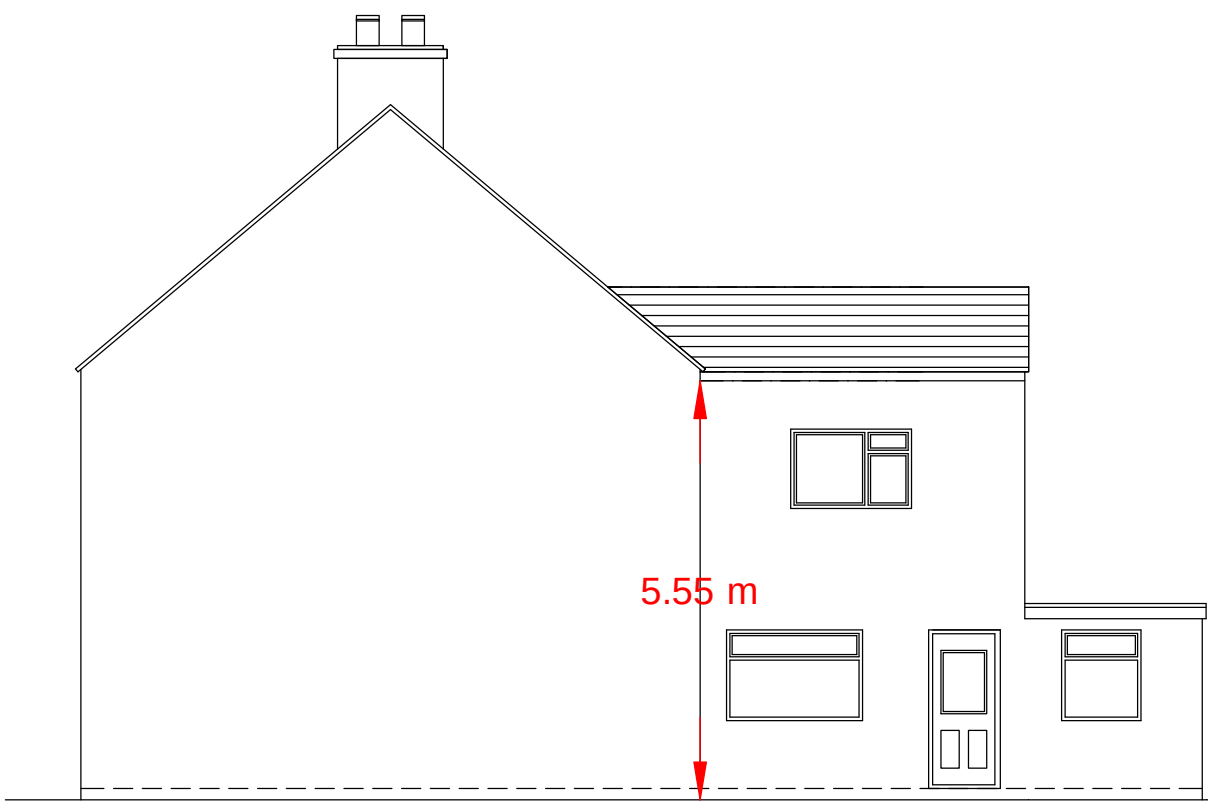
South-east elevation
