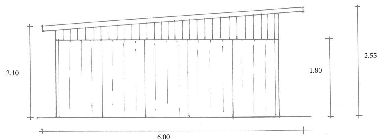
SIDE ELEVATION
