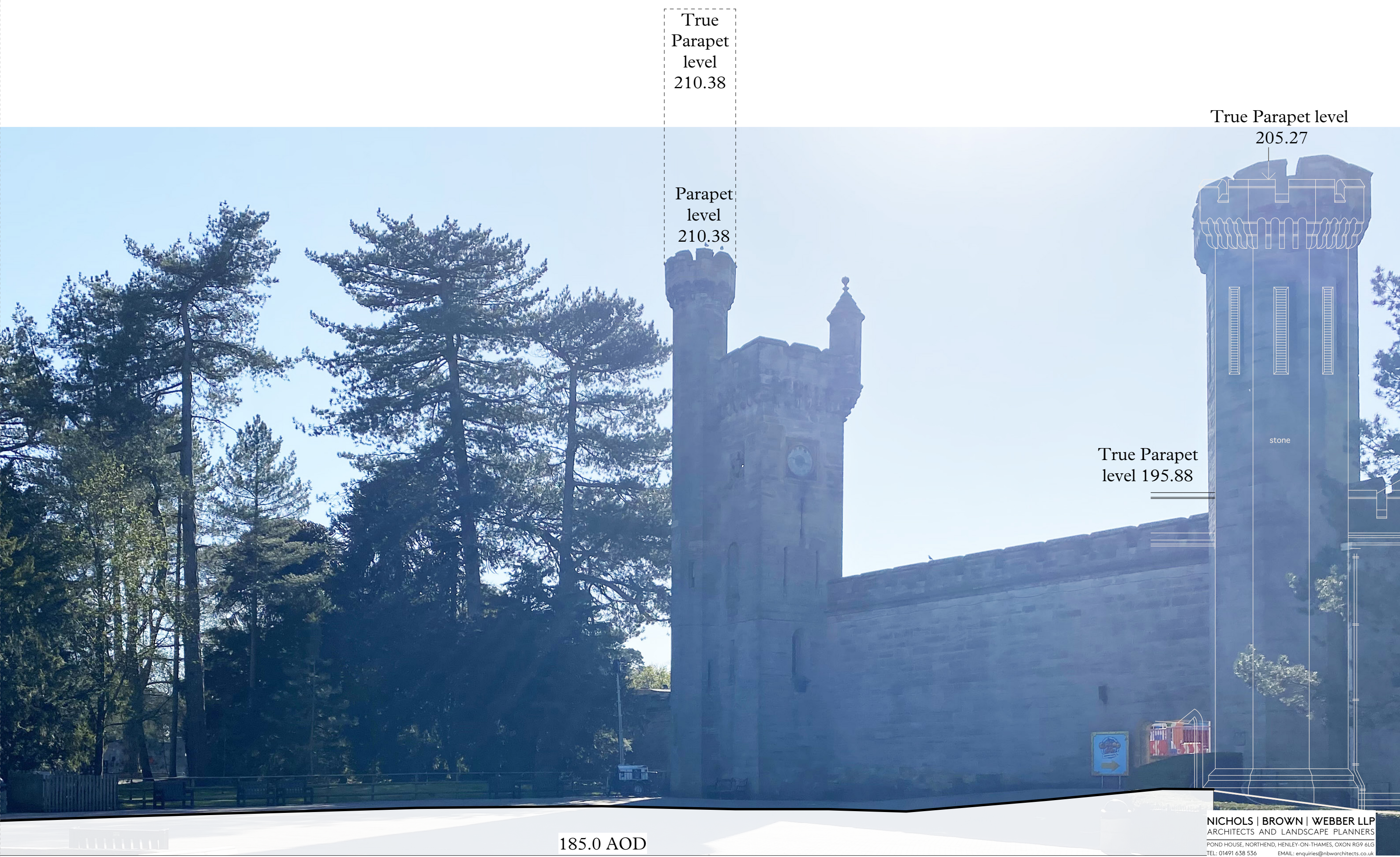
Existing Site Section in Context. (Scale is true at section in white above and through tower at right)
