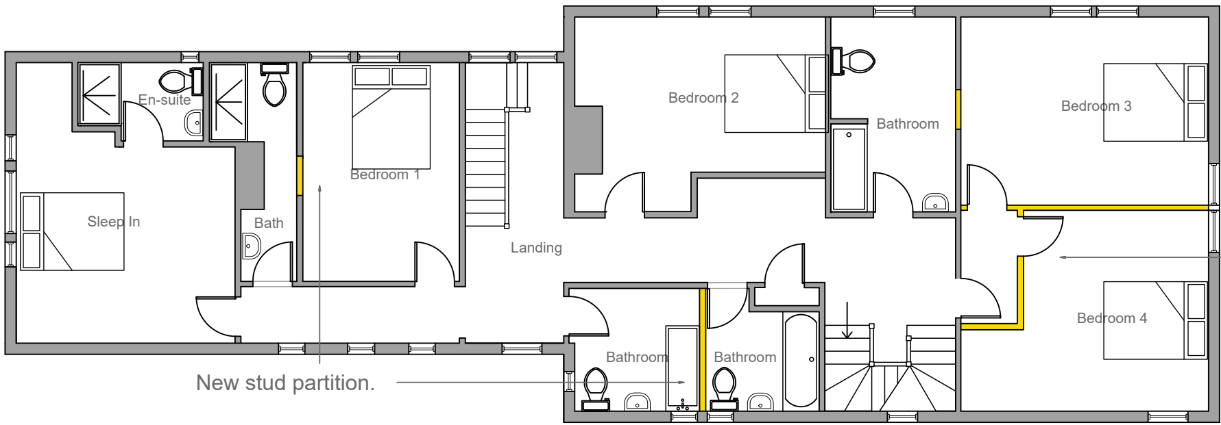
First Floor
