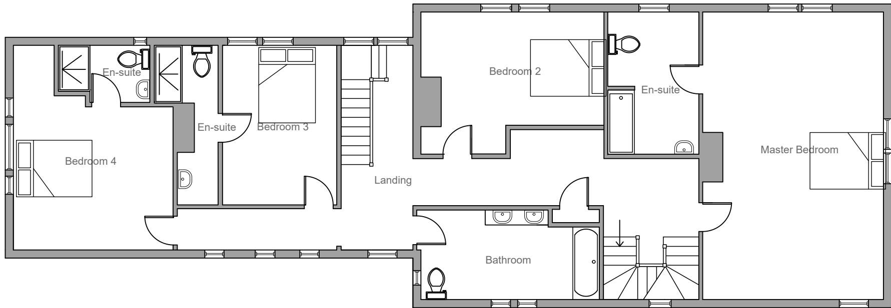
First Floor
