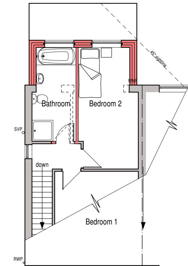
Part First Floor
