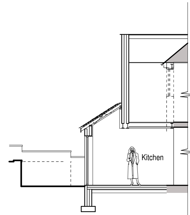
Typical Section (North East)
