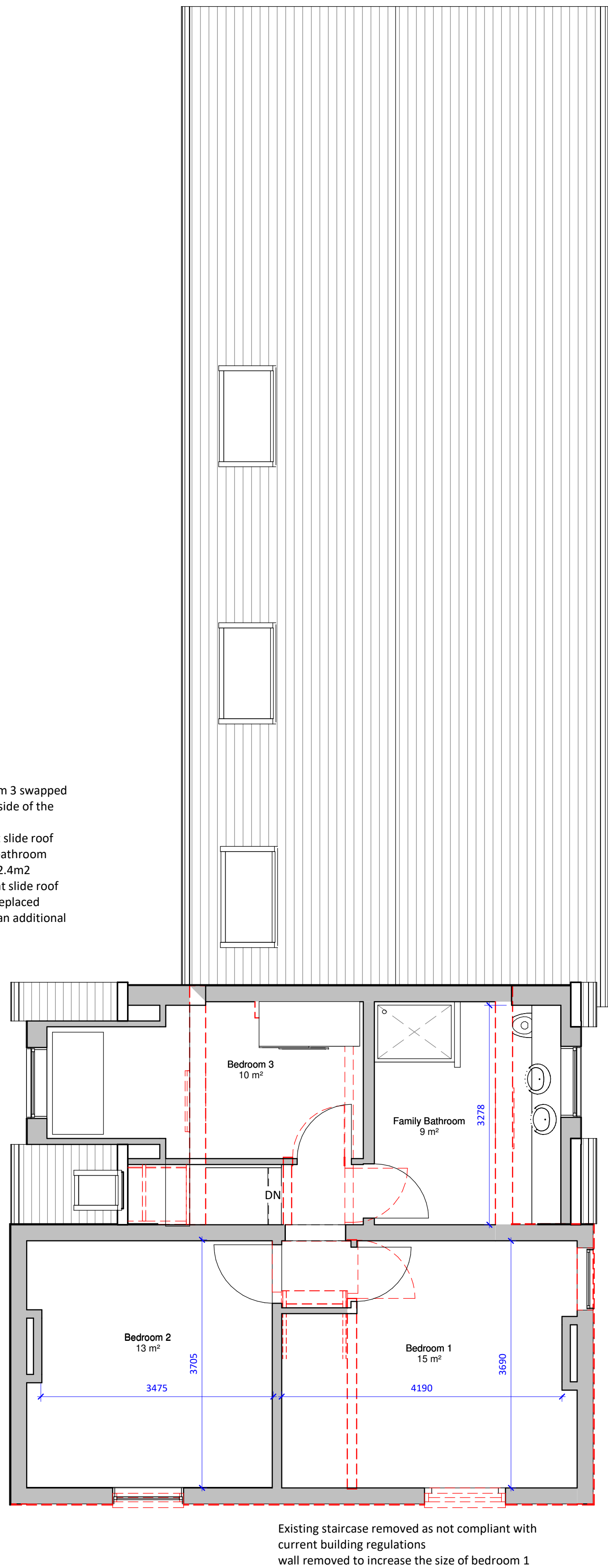
1.0 FF - Proposed 1 : 50
