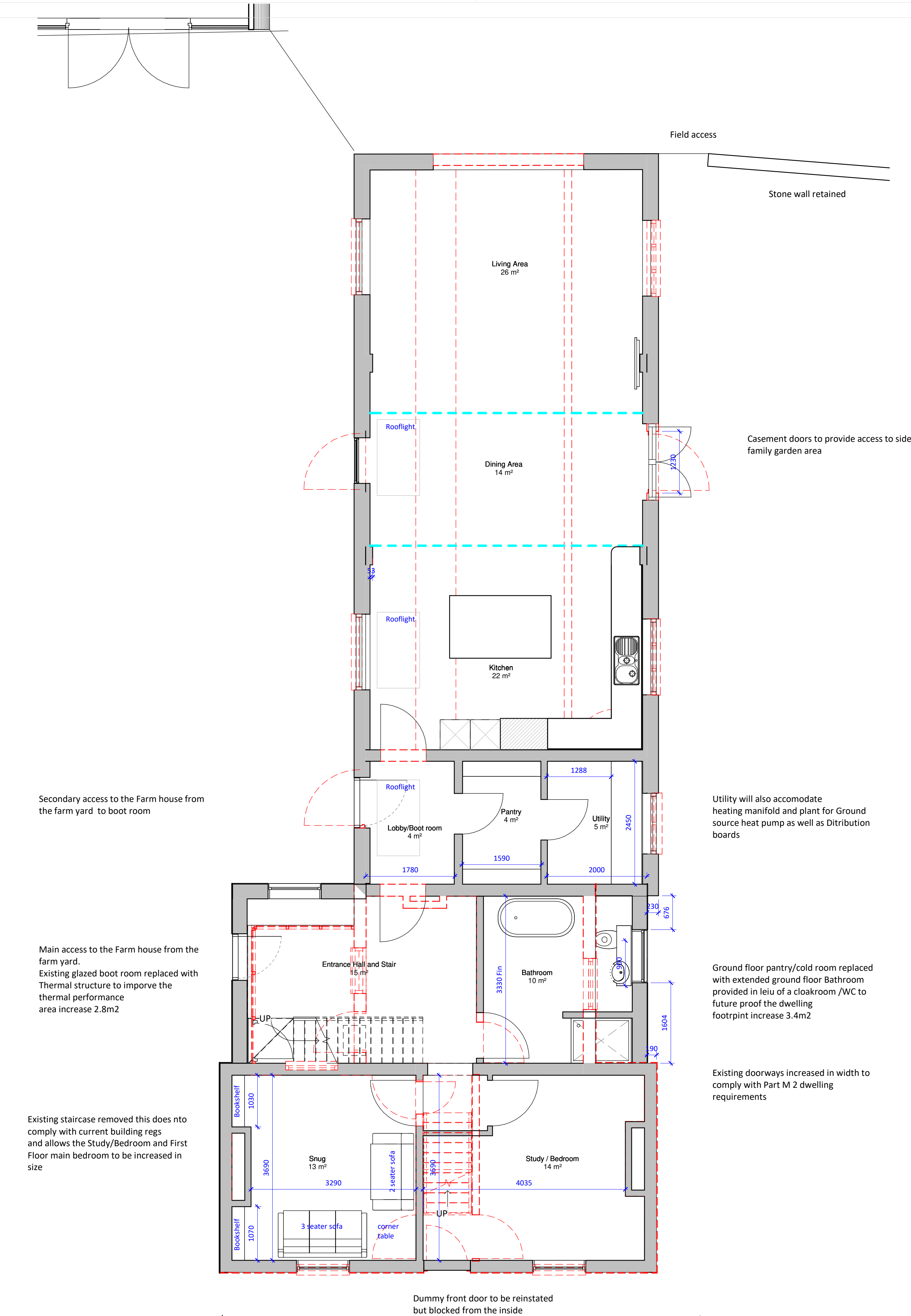
0.0 GF - Proposed 1 : 50
