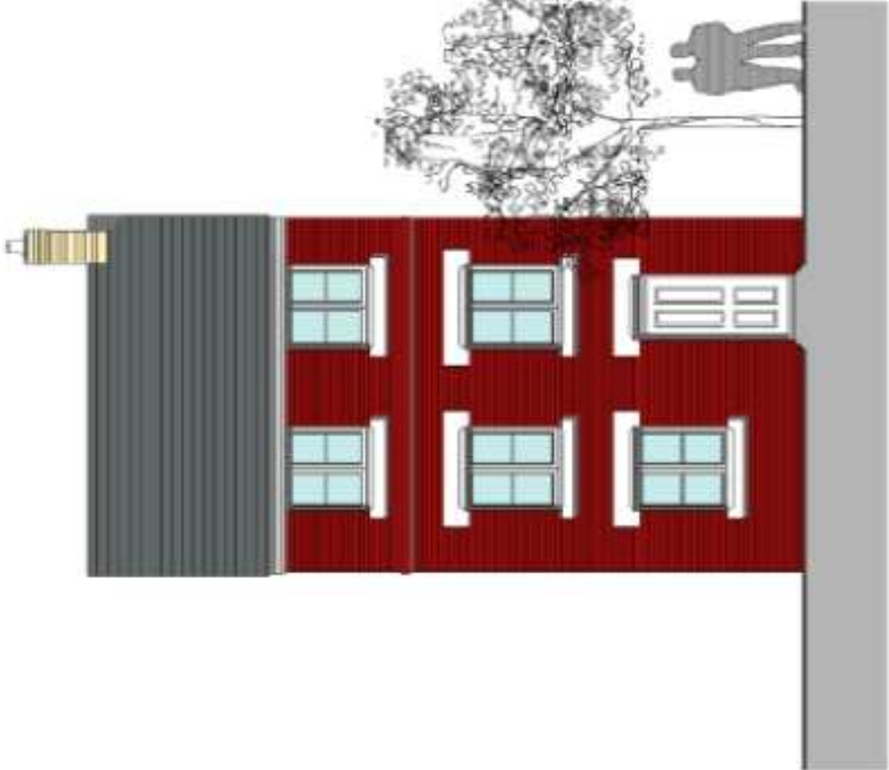
FRONT ELEVATION
