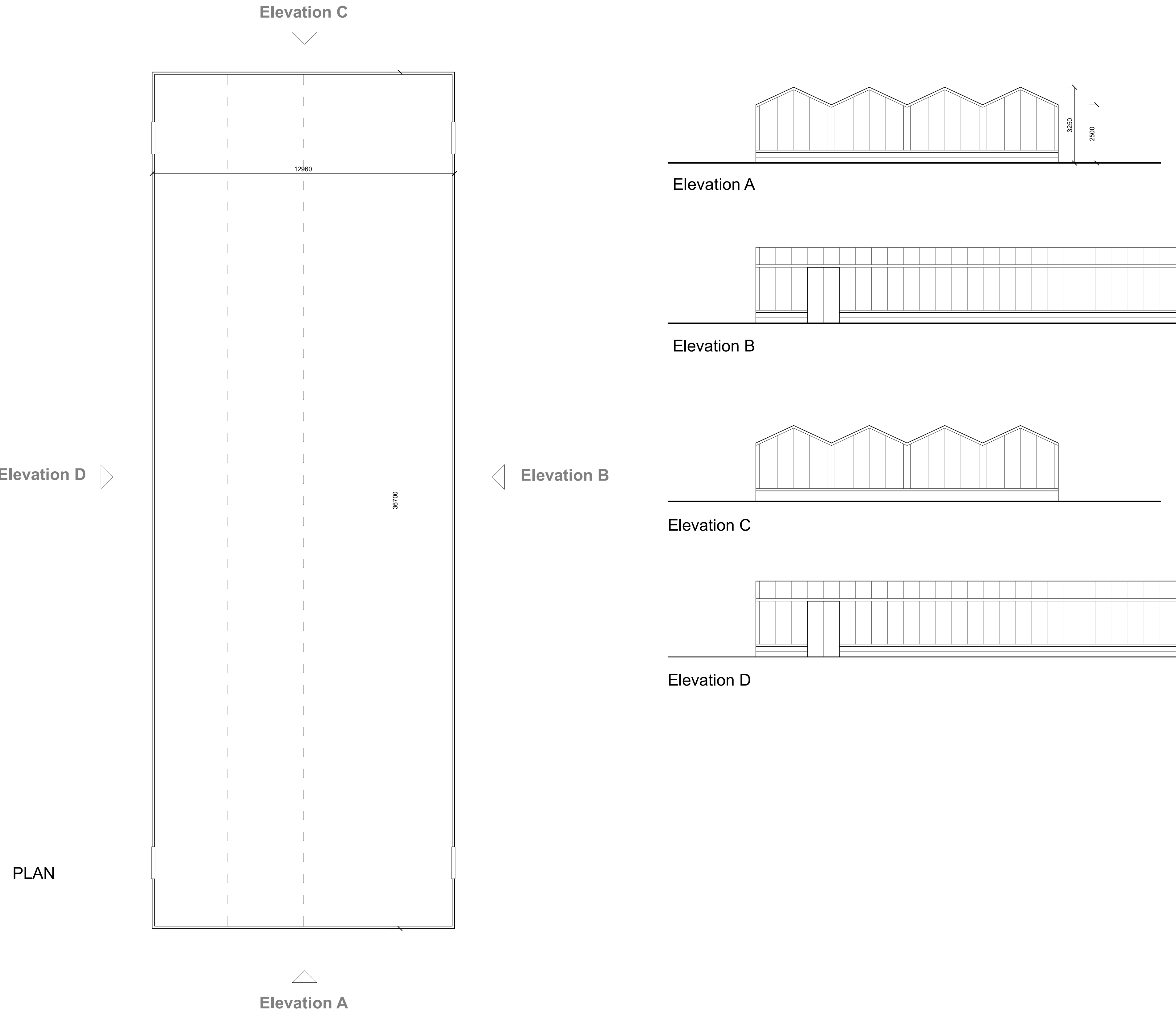
EXISTING GREENHOUSE 1 (As noted on site plan drawing PL-01A) 1:100
