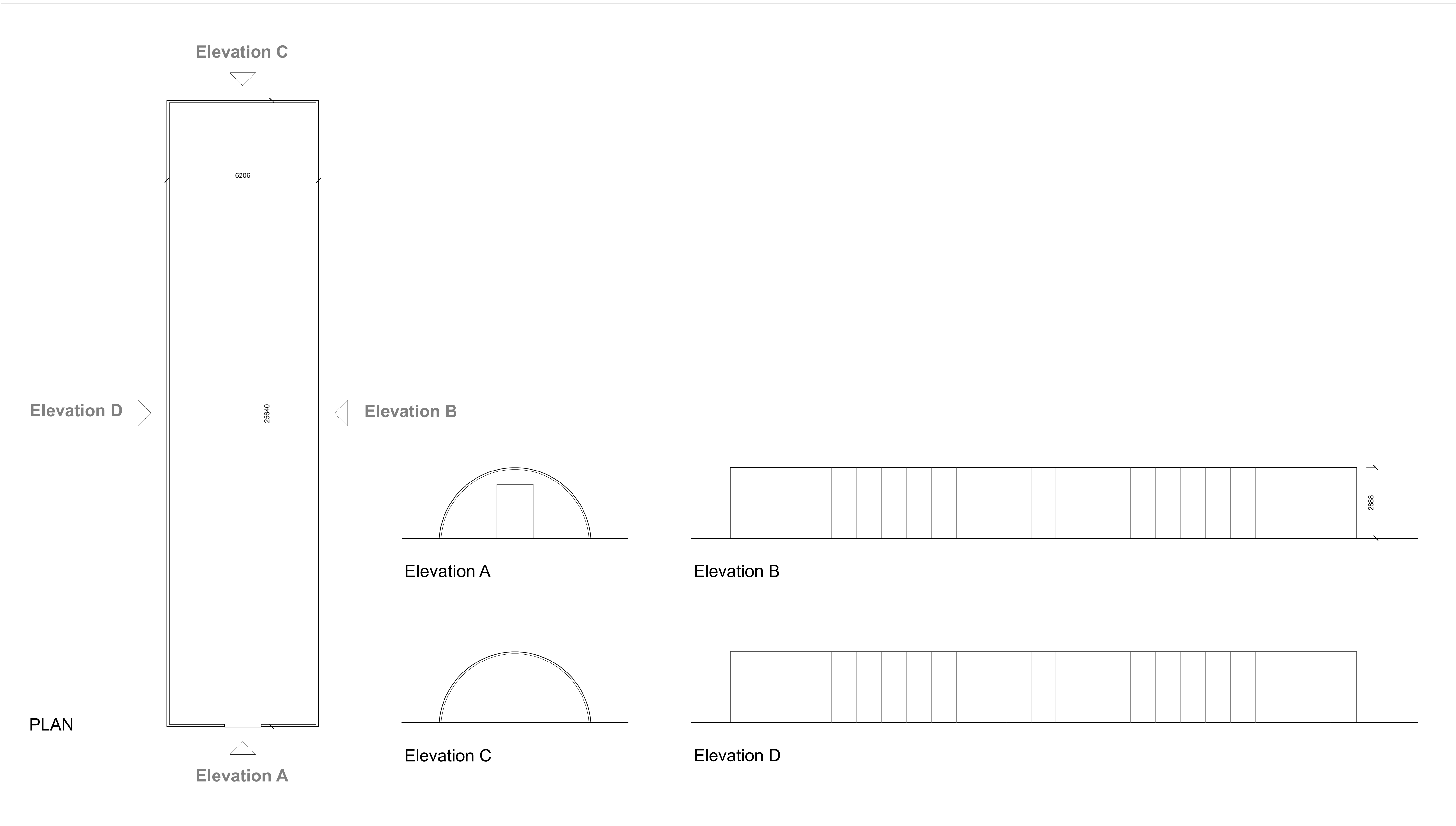
EXISTING POLYTUNNEL 1 (As noted on site plan drawing PL-01A) 1:100
