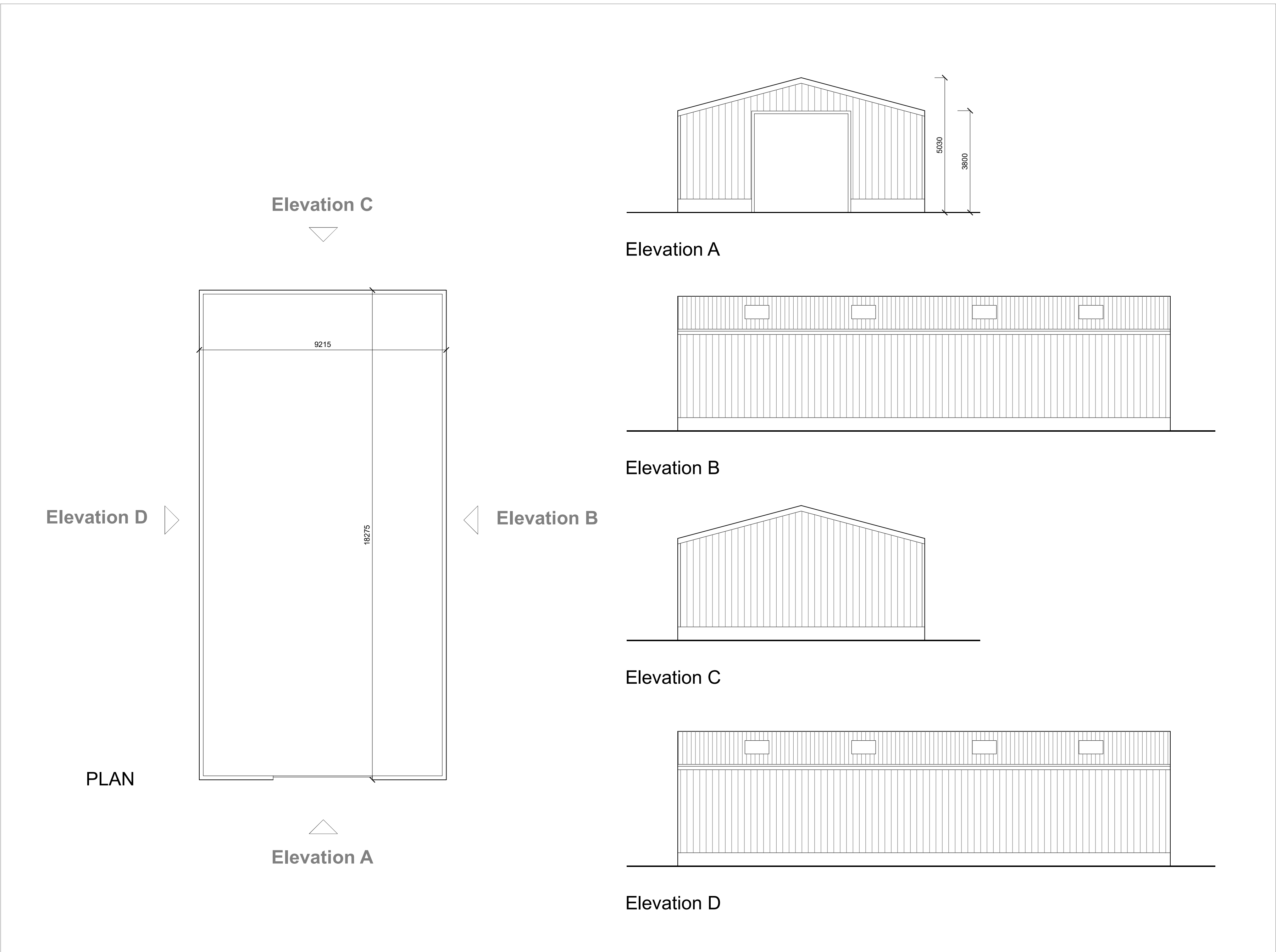
EXISTING SHED (As noted on site plan drawing PL-01A) 1:100
