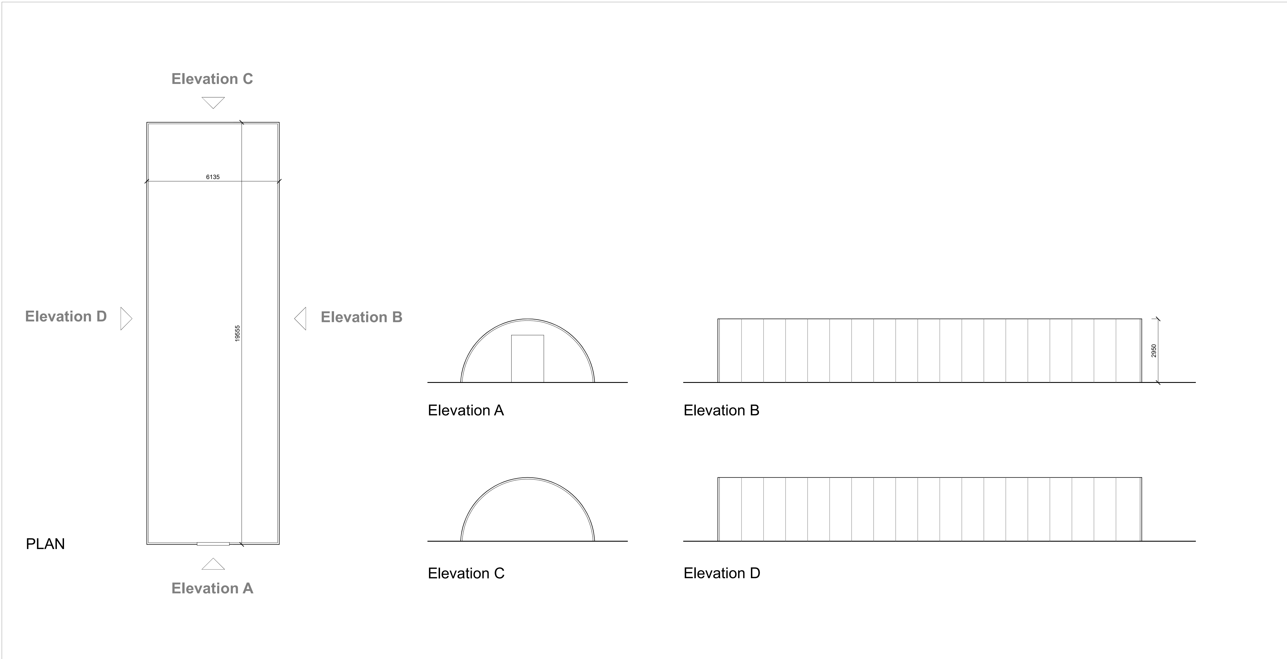
EXISTING POLYTUNNEL 2 (As noted on site plan drawing PL-01A) 1:100
