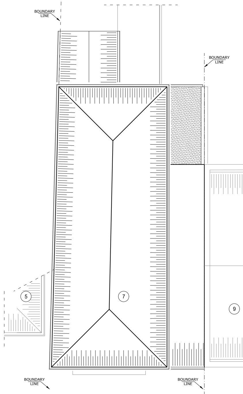
EXISTING ROOF PLAN SCALE: 1/100 @A3
