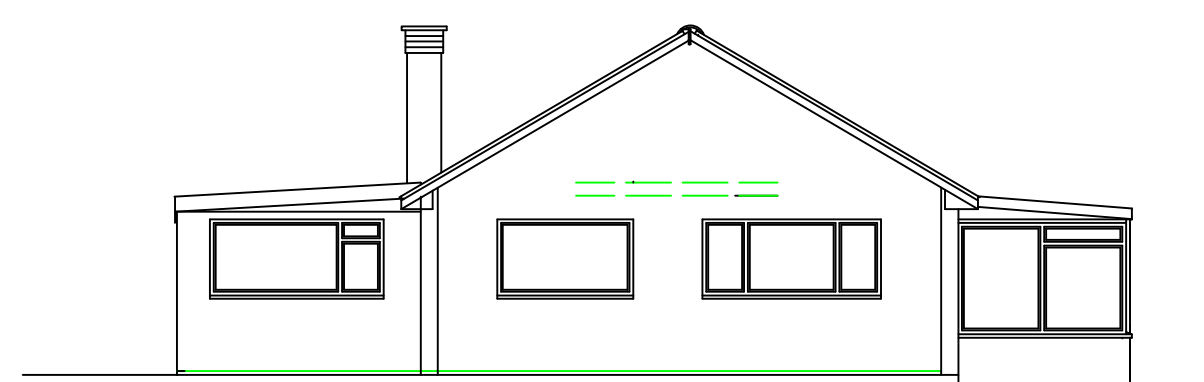
REAR NORTH WEST ELEVATION
