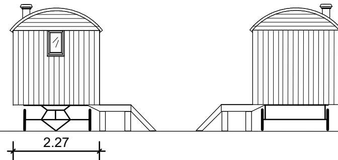
PROPOSED SIDE ELEVATIONS
