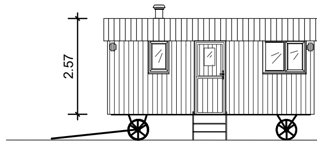
PRPOSED FRONT ELEVATION
