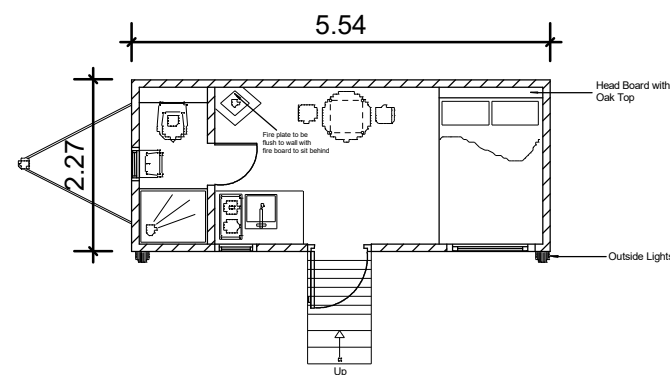
PROPOSED FLOOR PLAN
