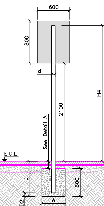
Typical Single Signage Pole Installation Detail
