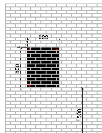
Typical Signage Wall Installation Details
