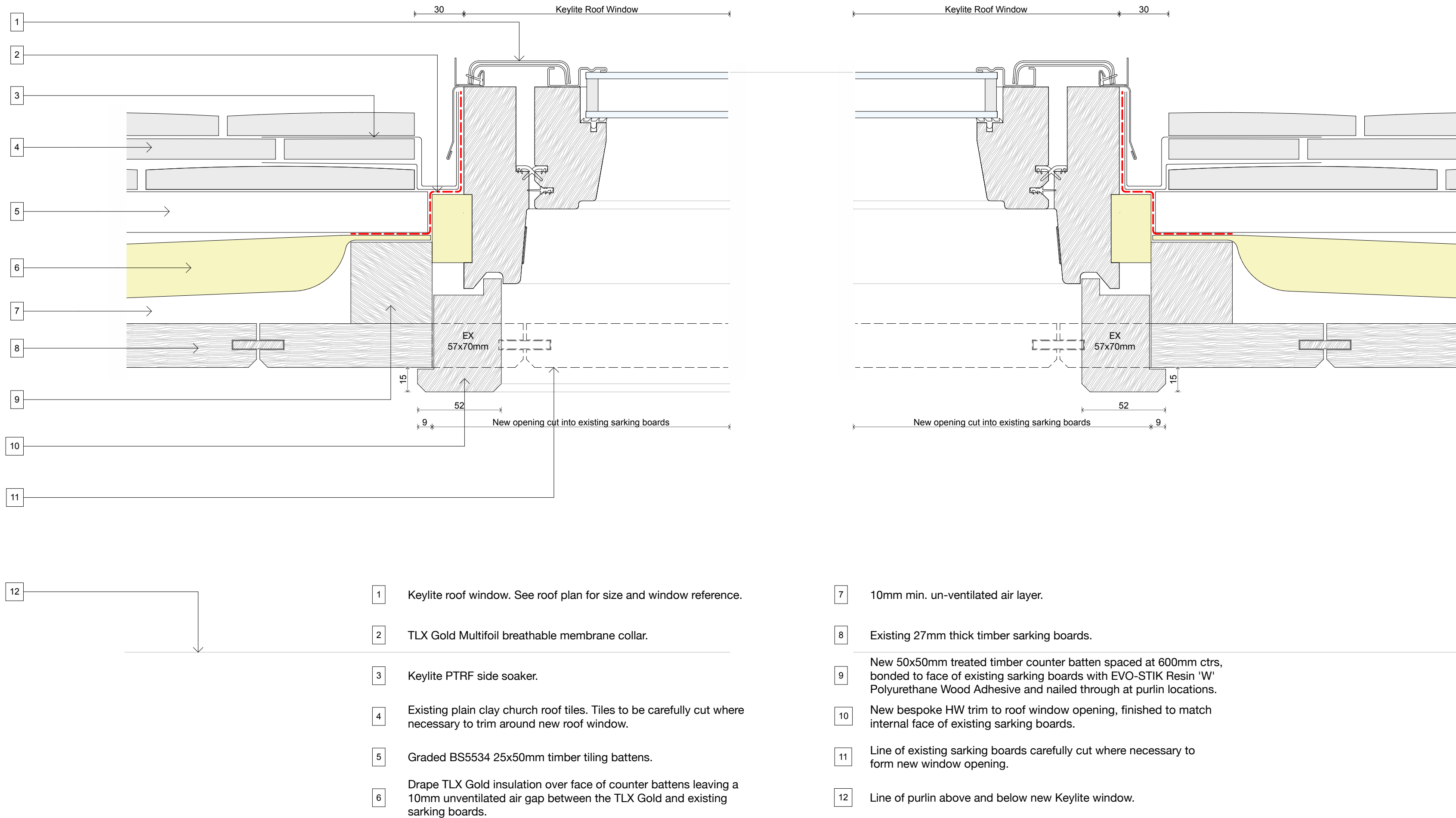
Roof Window Jamb Detail
