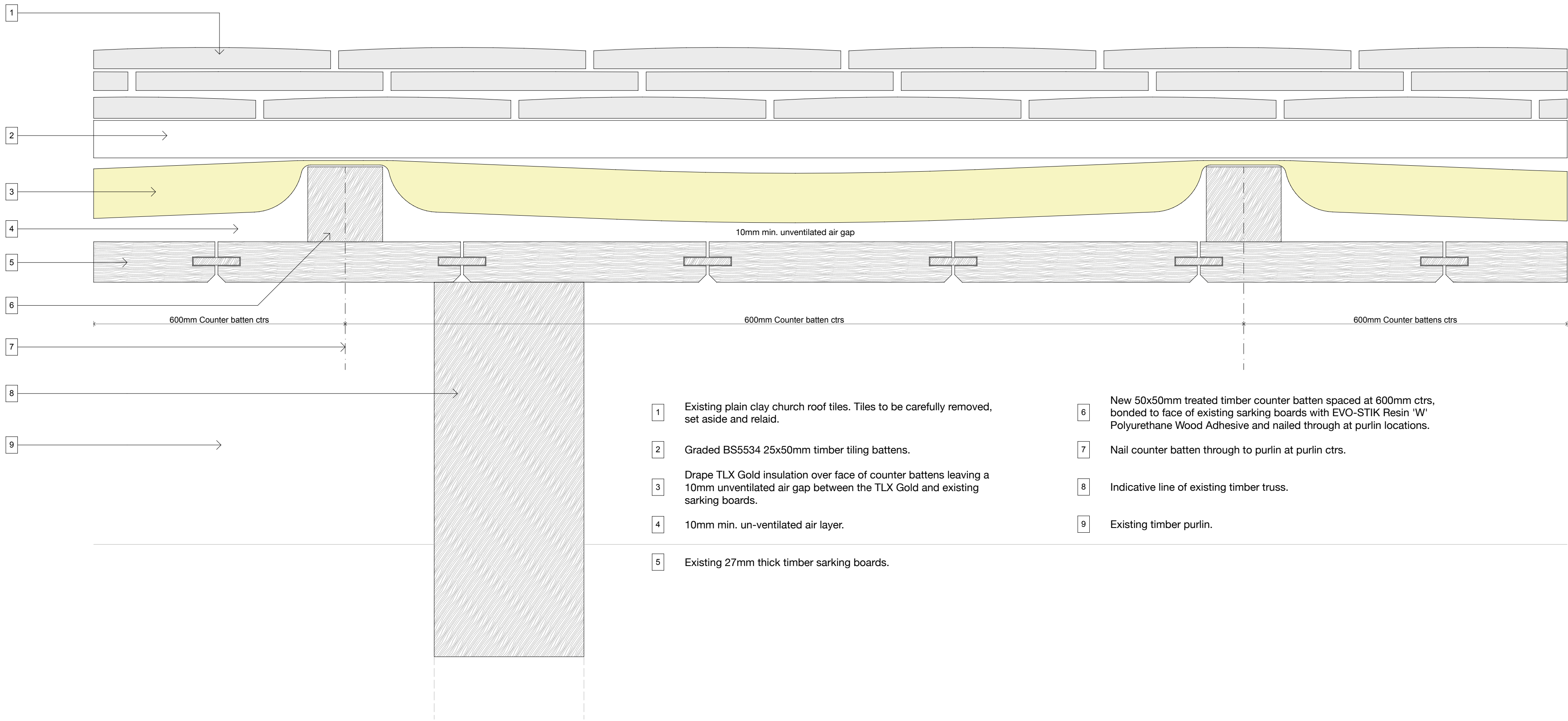
Typical Roof Cross Section
