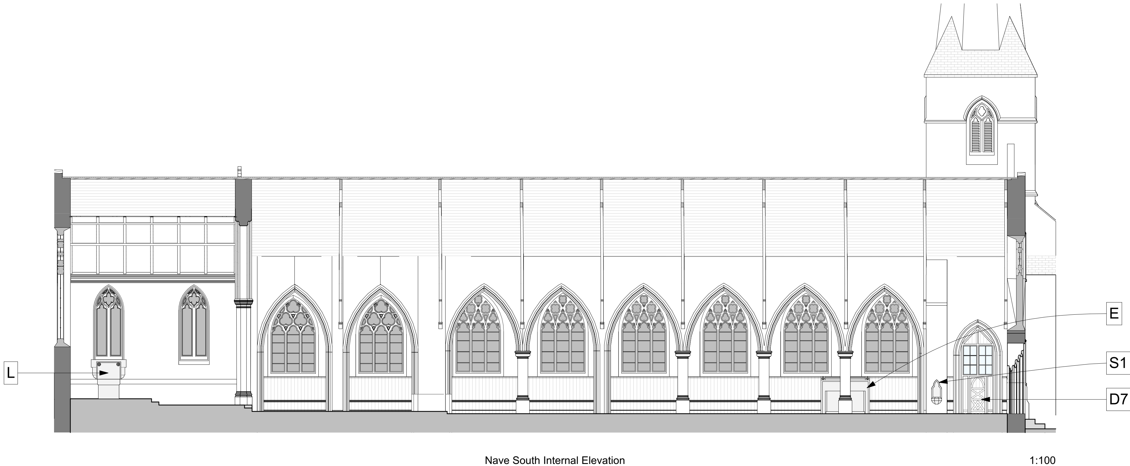
Nave South Internal Elevation
