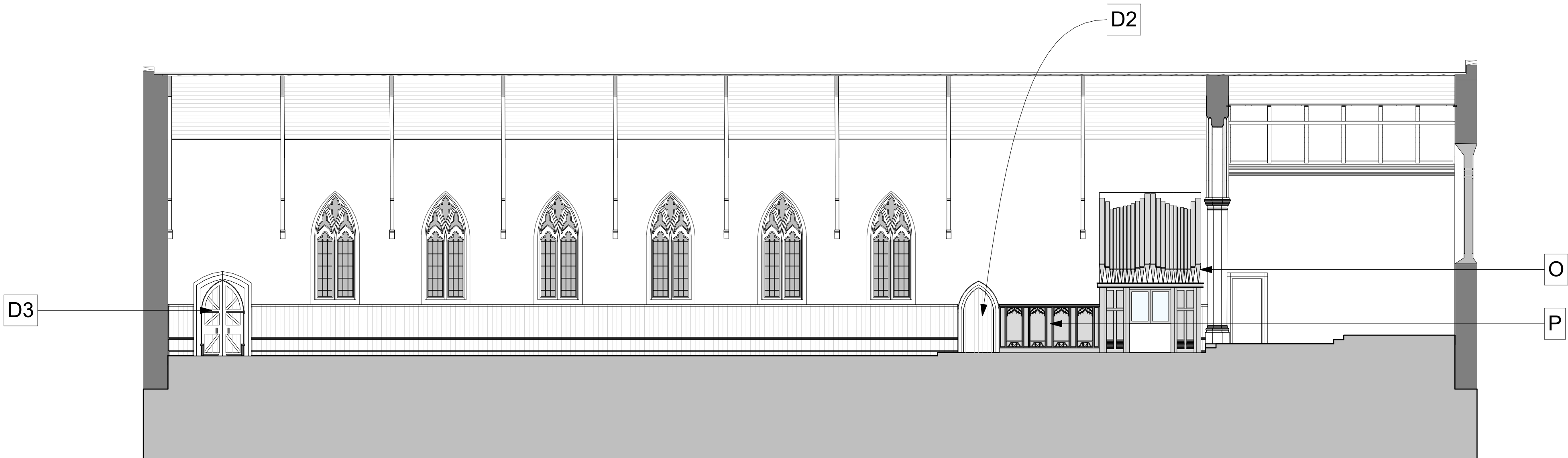
Nave North Internal Elevation
