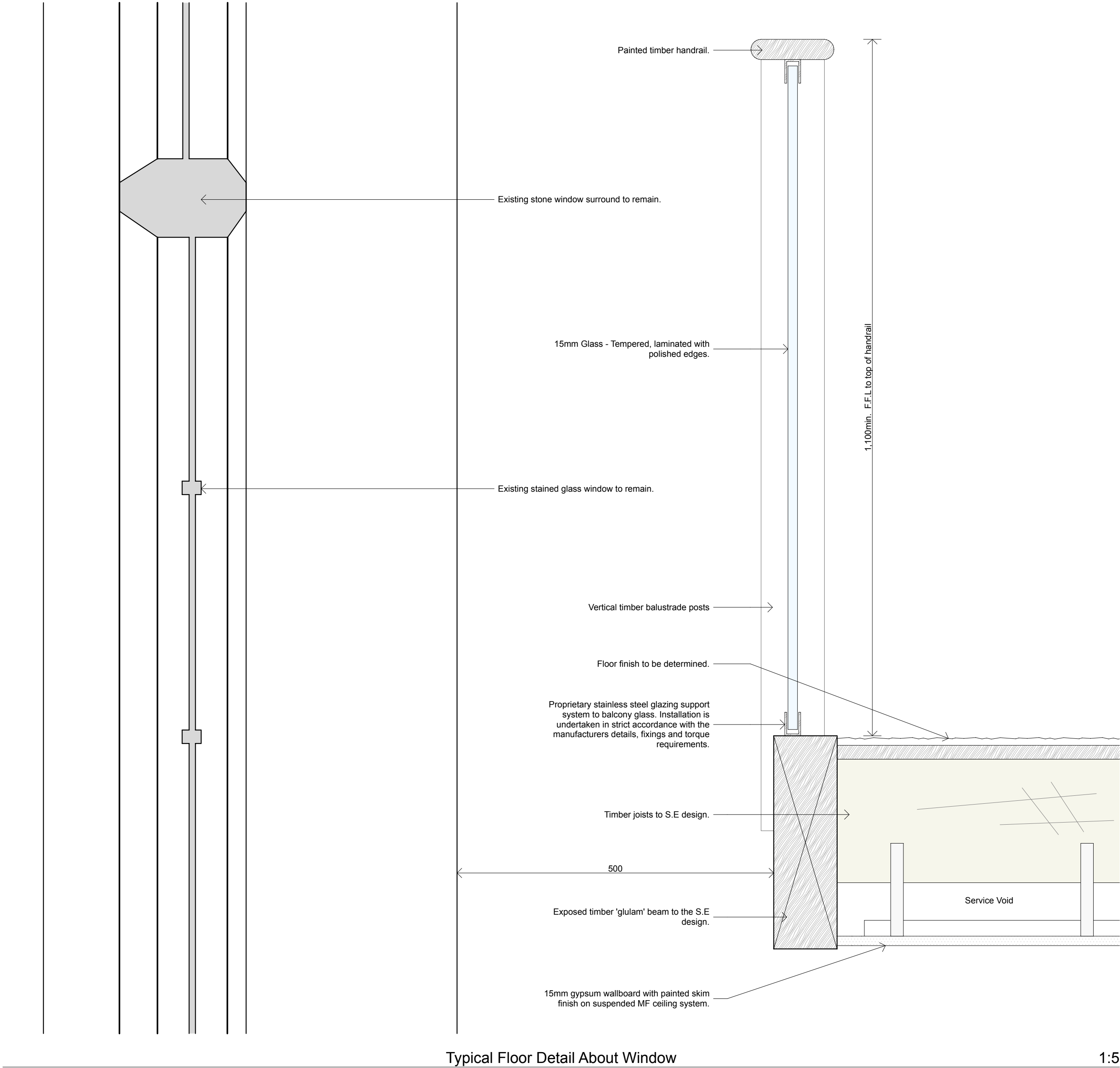
Typical Floor Detail About Window
