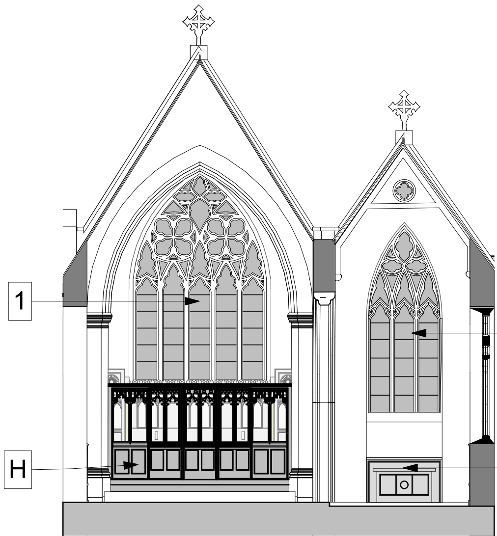
Nave East Internal Elevation 1:100
