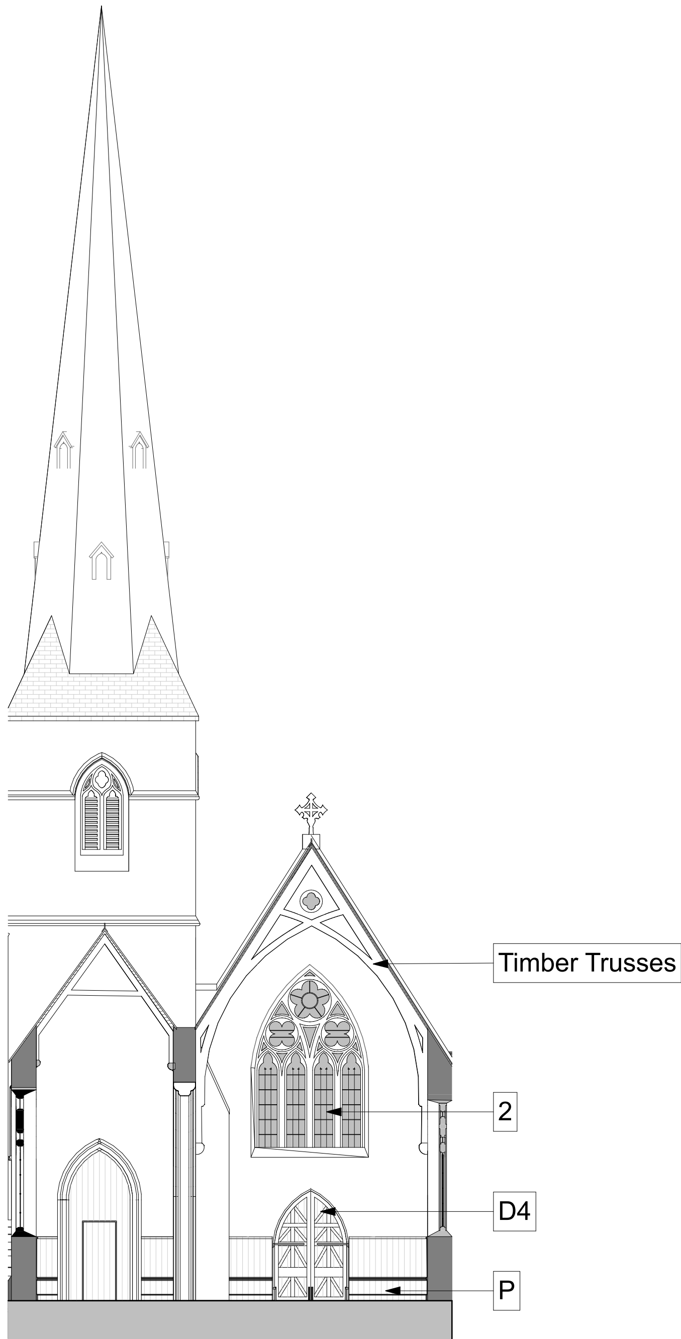
Nave West Internal Elevation 1:100
