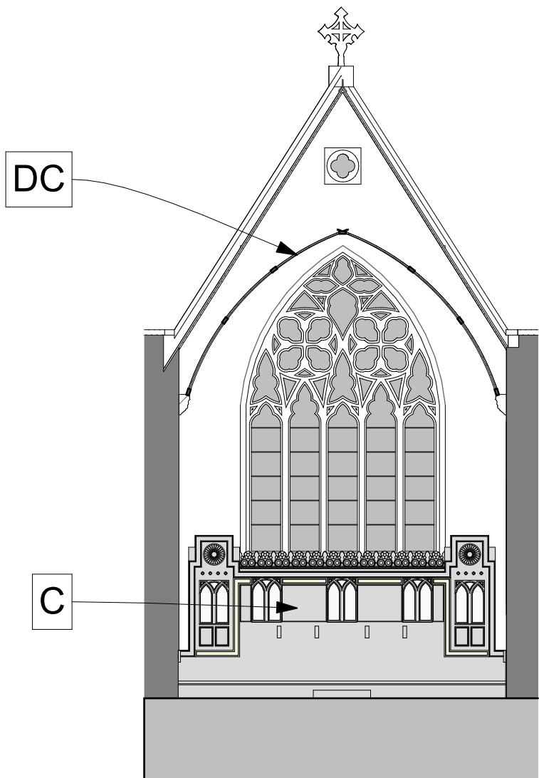
Sanctuary East Internal Elevation
