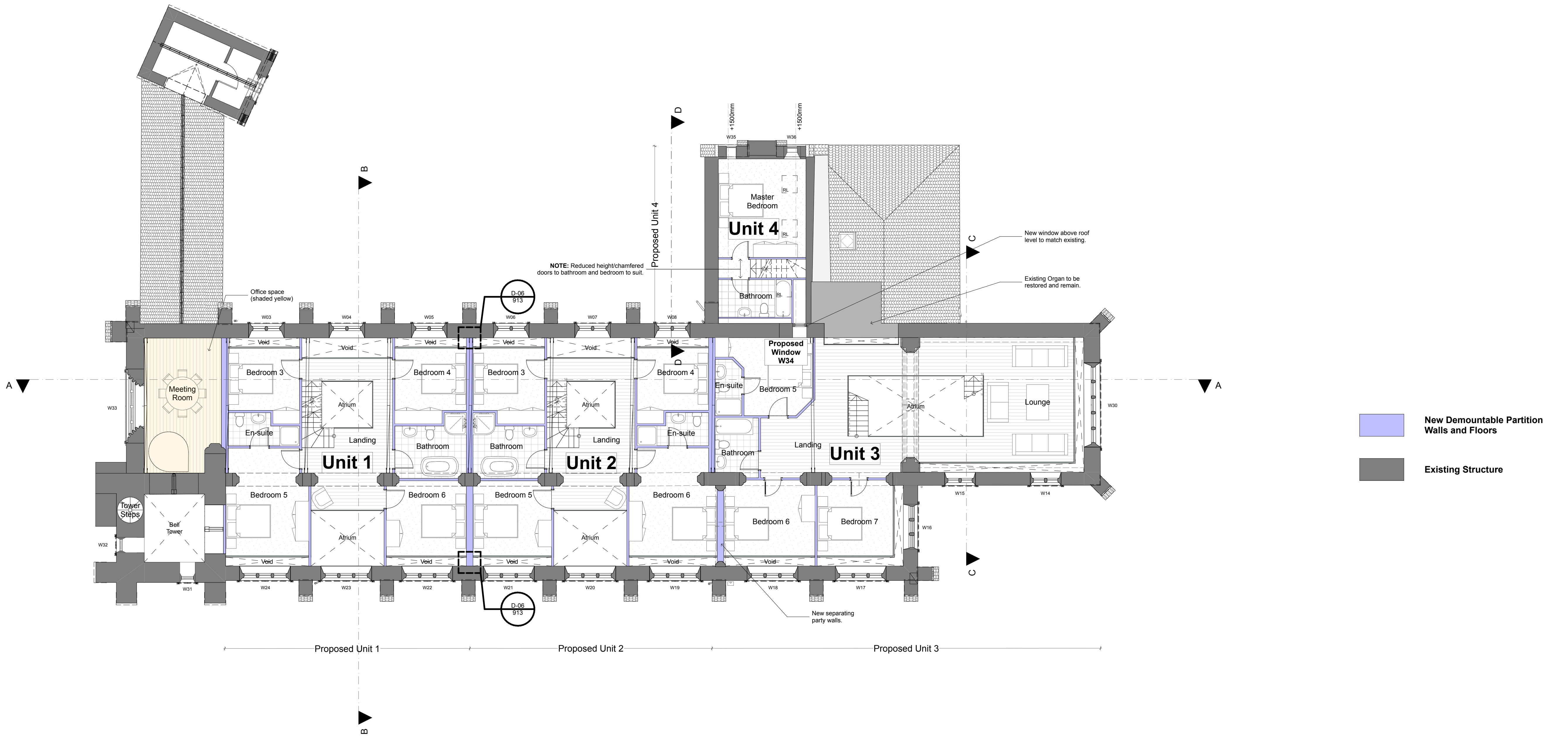
Proposed First Floor Plan
