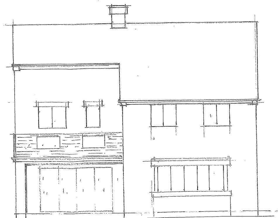
AS PROPOSED REAR ELEVATION - SOUTH
