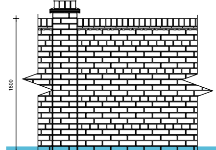
ELEVATION DETAIL TO 1.8m HIGH SCREEN WALL (BRICK)
