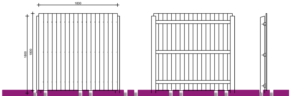
ELEVATION DETAIL TO 1.8m HIGH CLOSE BOARD FENCE
