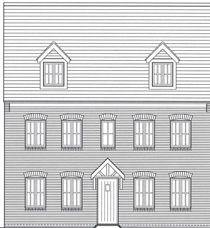
FRONT ELEVATION 'Village Style'
