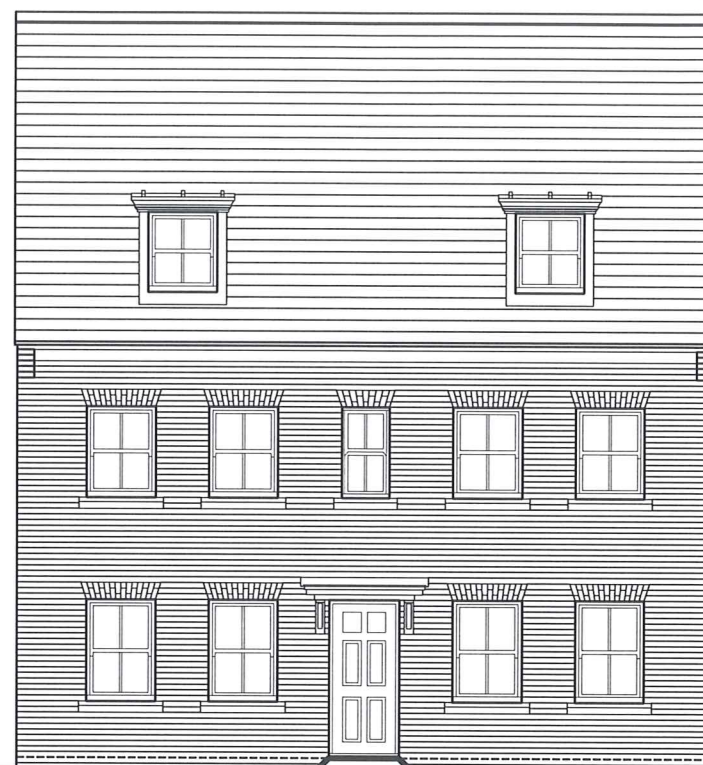
FRONT ELEVATION 'Classic Style'
