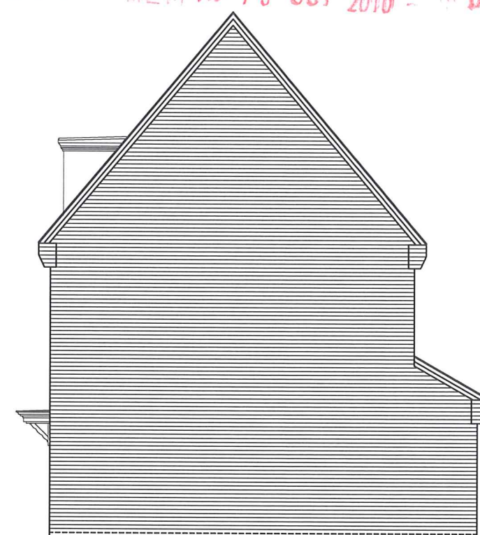
SIDE ELEVATION
