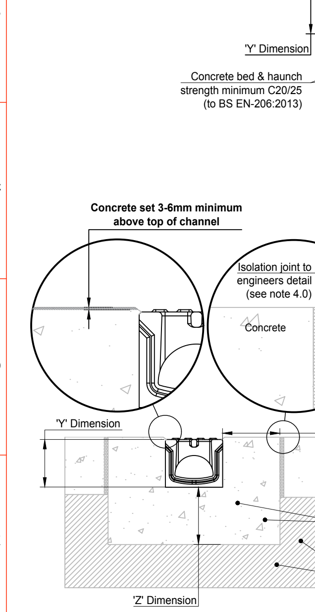
1 : 10 ACO KerbDrain KDHB Concrete Pavement
