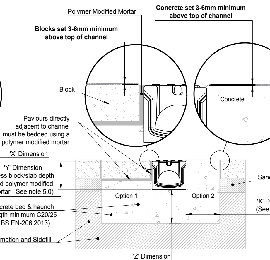
1 : 10 ACO KerbDrain KDHB Block Pavement (Option 1 and 2)
