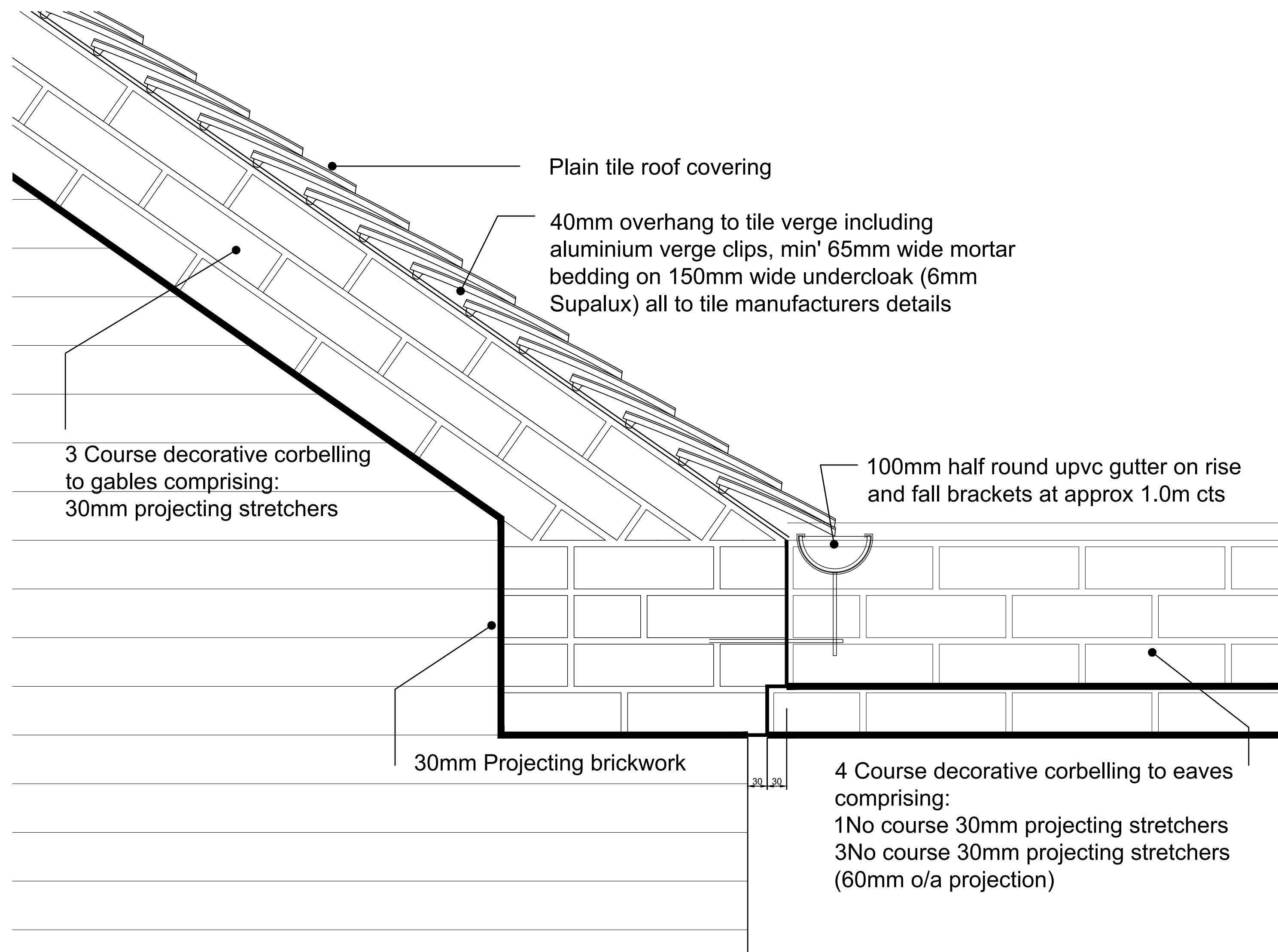
BRICK CORBEL DETAILS (SCALE 1:5)
