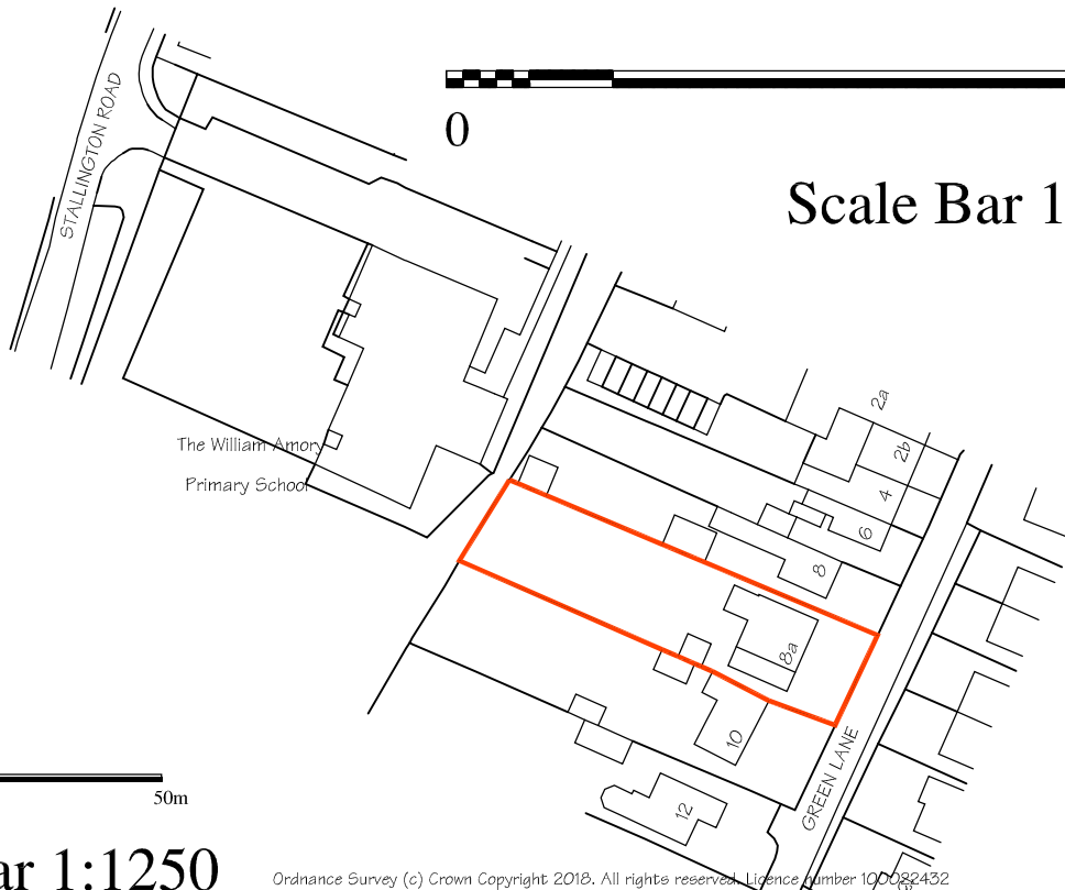
Location Plan 1:1250
