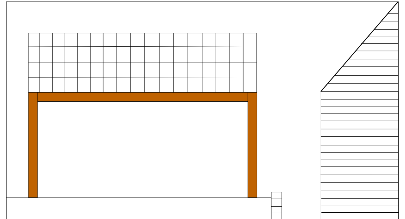
Proposed elevation Scale = 1:50
