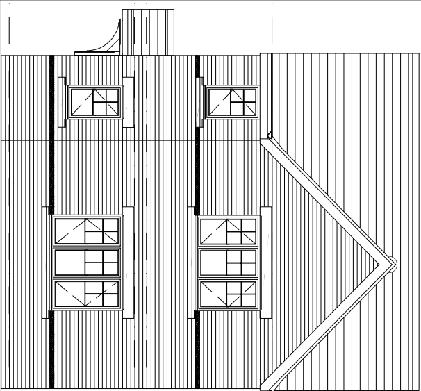
Front Elevation
