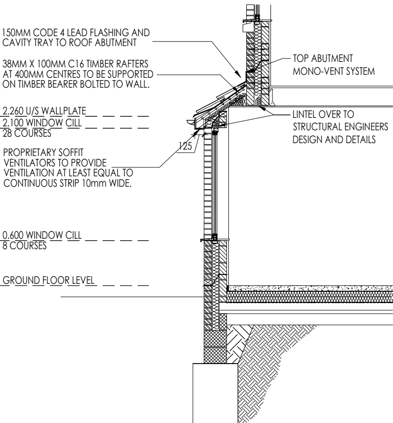
SECTION THROUGH CANOPY A Scale 1:50
