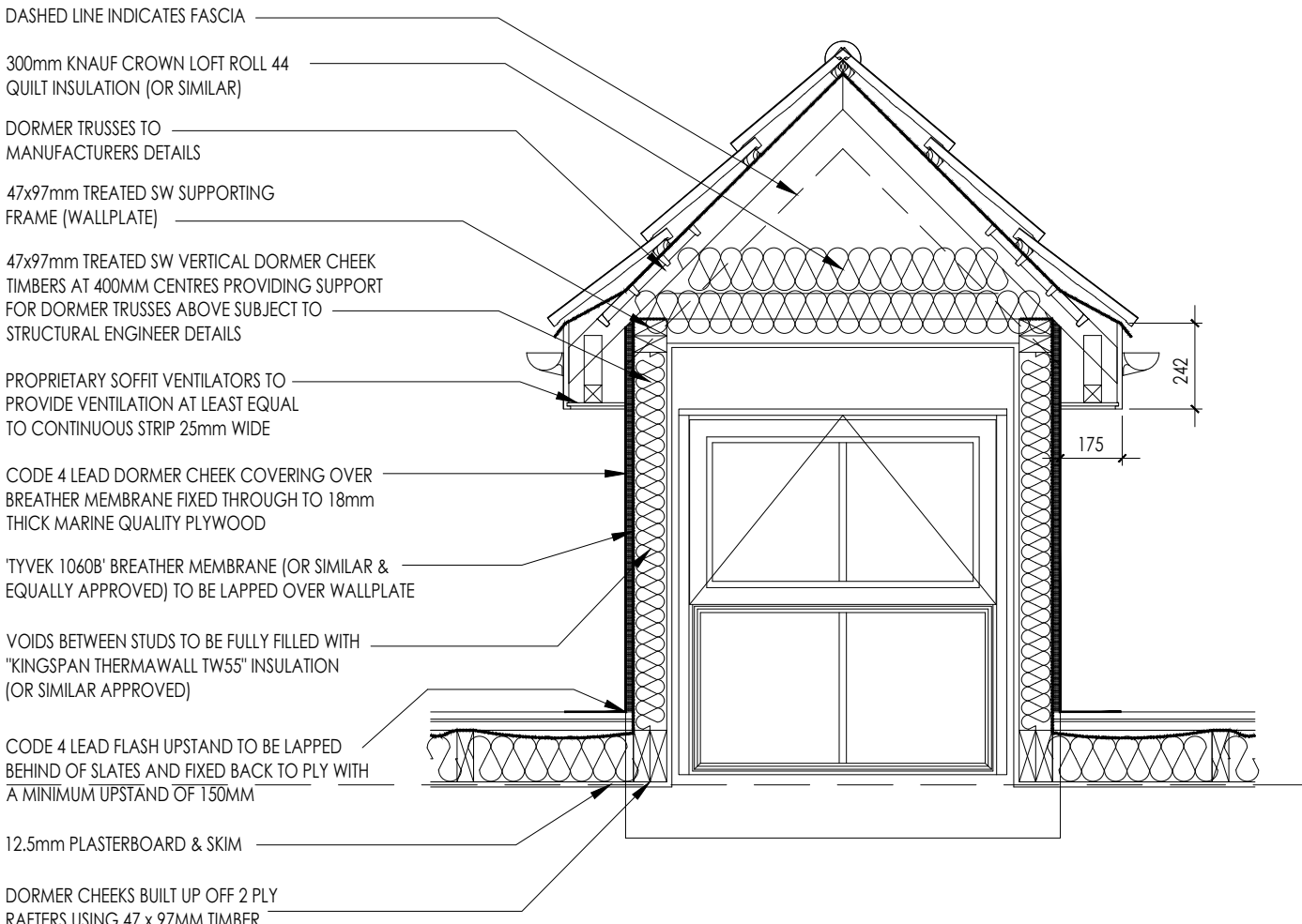
DORMER SECTION
