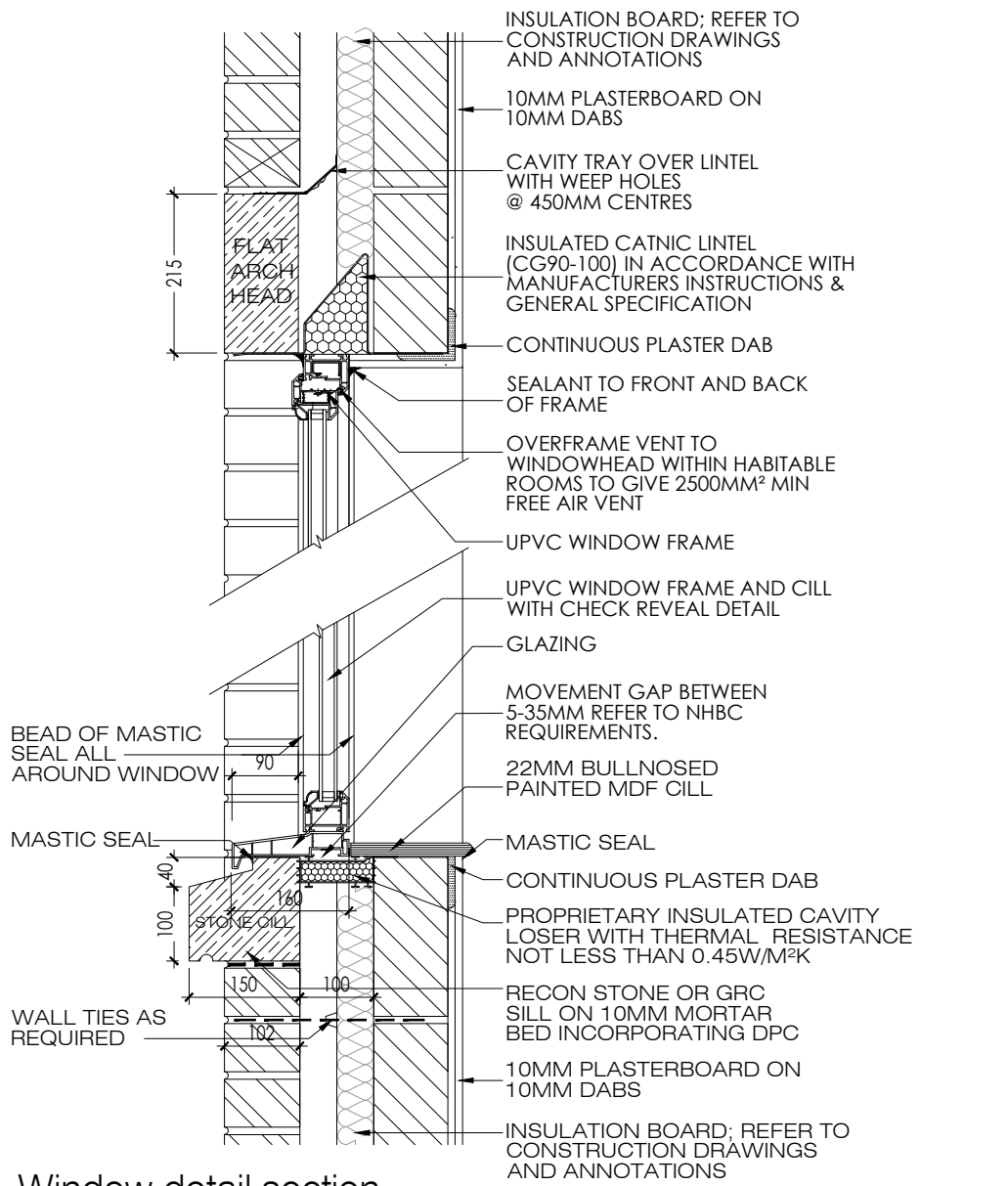
Window detail section
