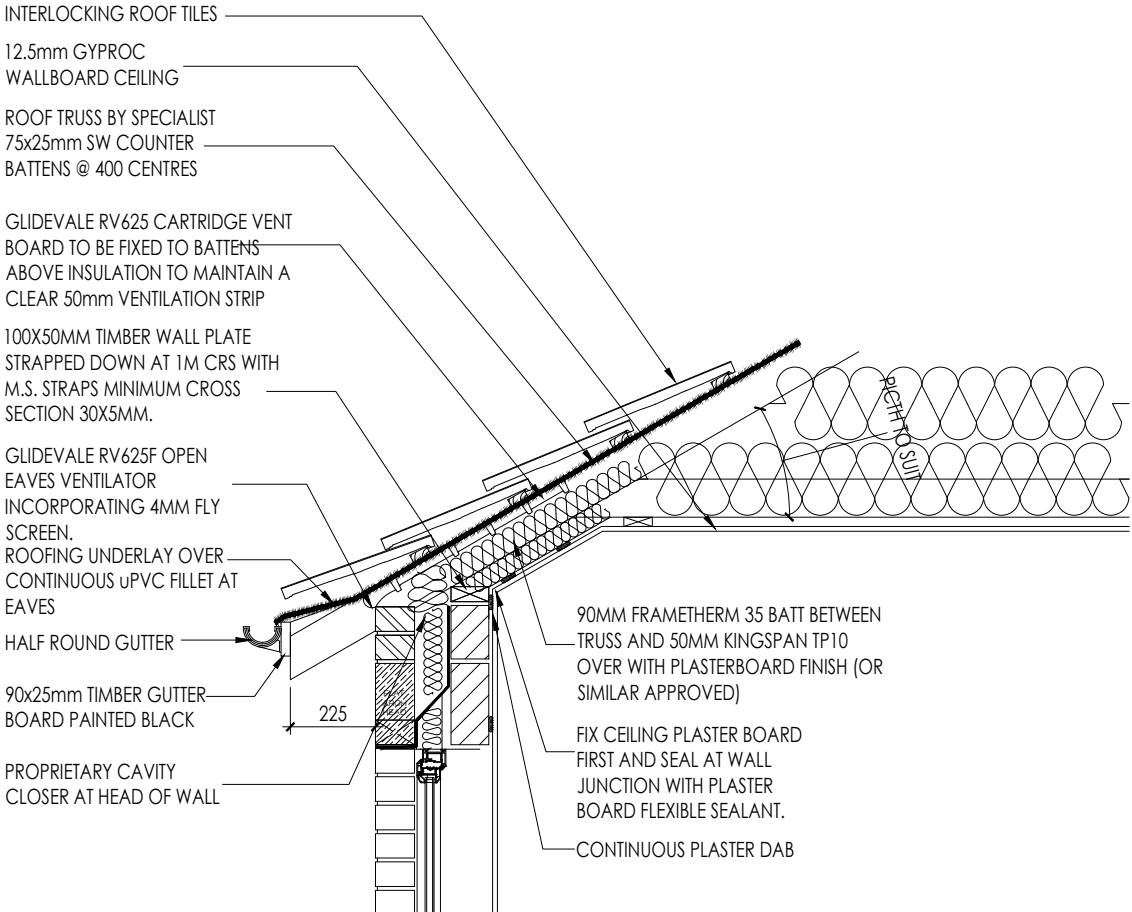
EAVES DETAIL Scale 1:20
