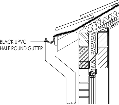
GUTTER DETAIL Scale 1:20
