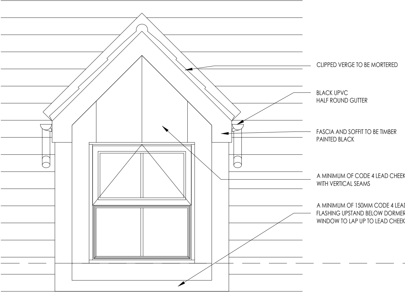
DORMER ELEVATION Scale 1:20
