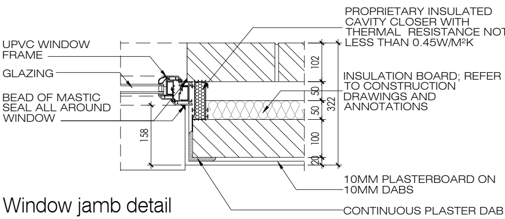
WINDOW DETAILS Scale 1:10
