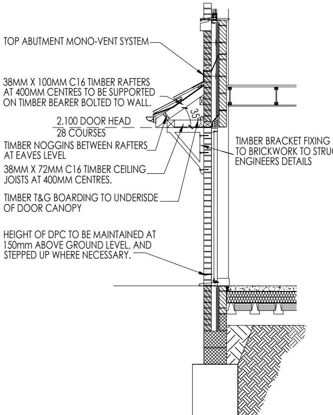
SECTION THROUGH CANOPY B Scale 1:50
