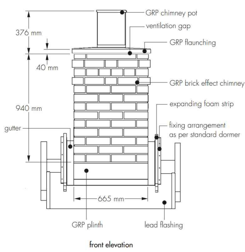
GRP CHIMNEY DETAIL Scale 1:20
