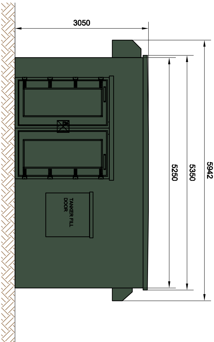
South East Elevation A 1:50
