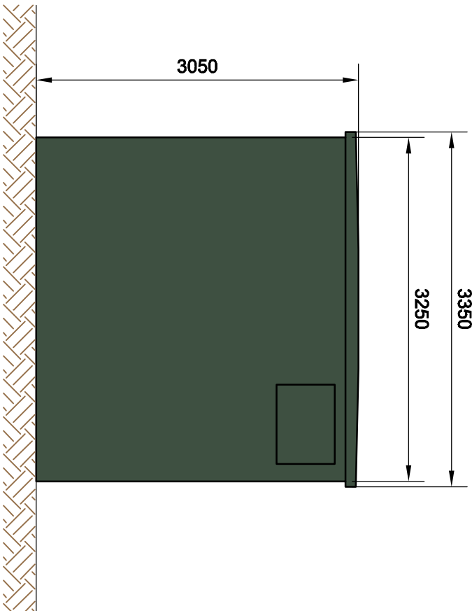
South West Elevation B 1:50
