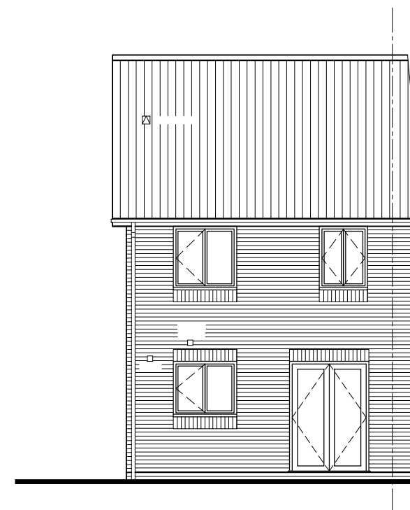
REAR ELEVATION
