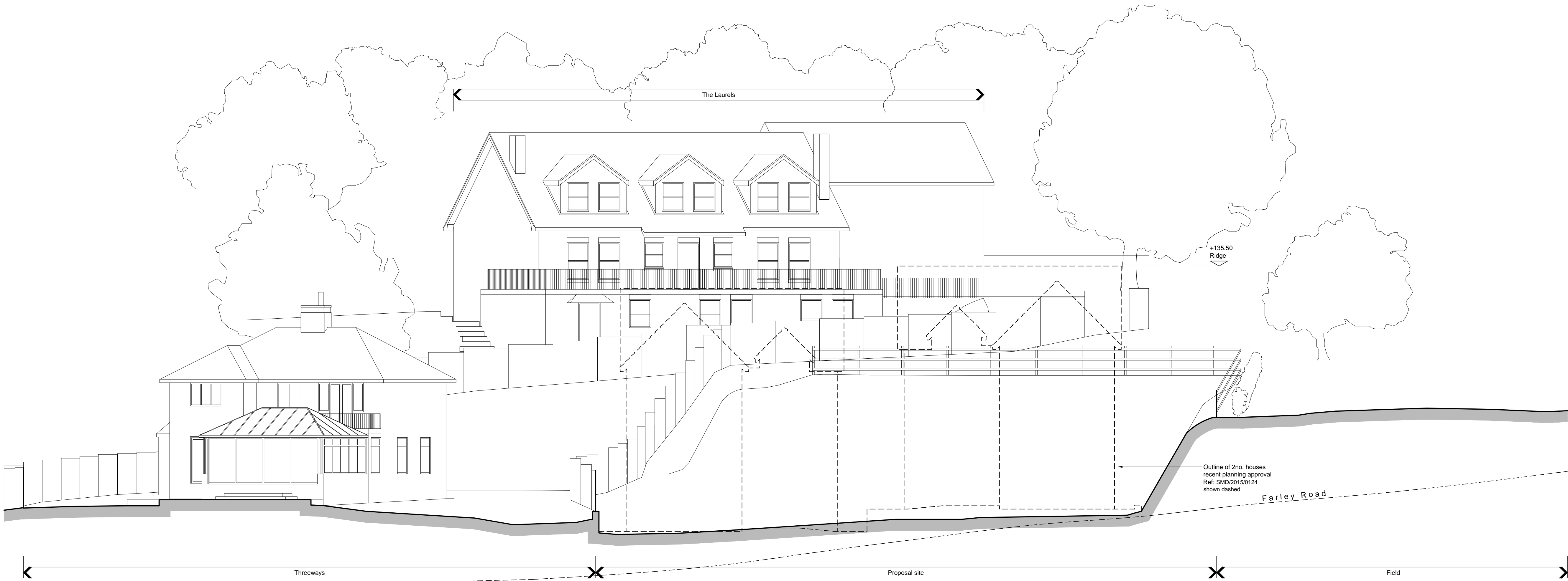
West Elevation (As Existing)
