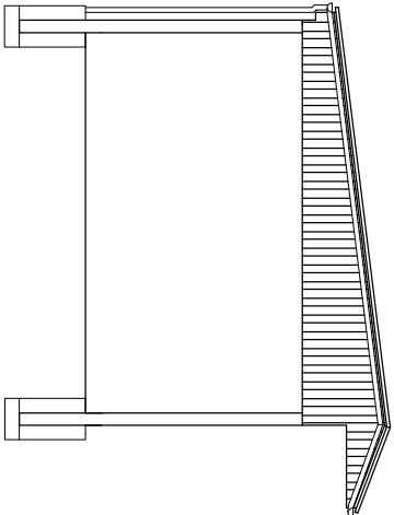
SIDE ELEVATION 1:100
