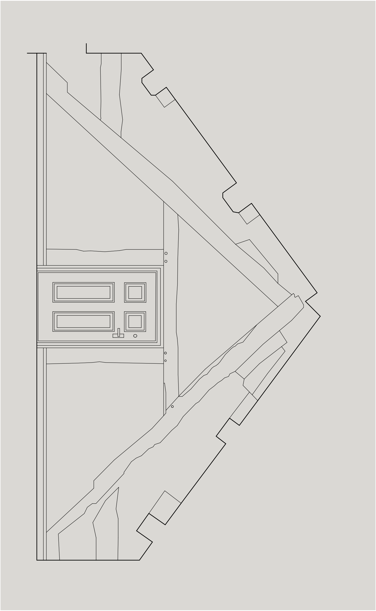
TRUSS A - VIEW 1 - Line Drawing
